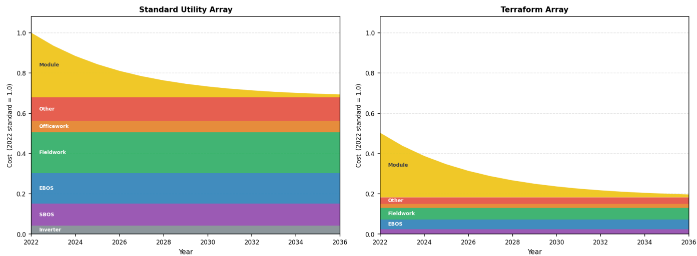
Solar Array Cost Breakdown Projection (Modules -20%/yr)
