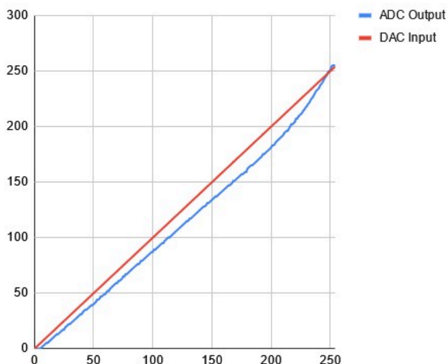
ADC Output vs. DAC Input (2.5 dB Attenuation)
