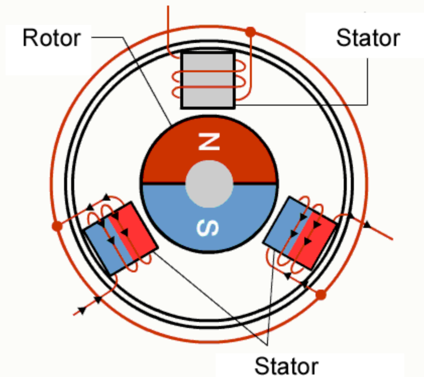
(Figure 2) This diagram shows how successive electromagnets are activated as north/south poles to push/pull the rotor. This is achieved through the use of the 6 motor FETs.
