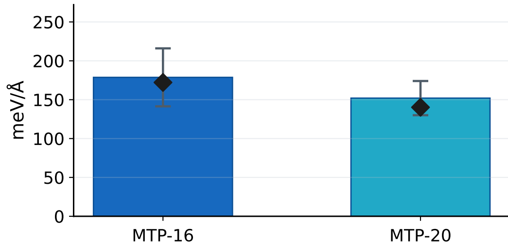
Forces MAE
