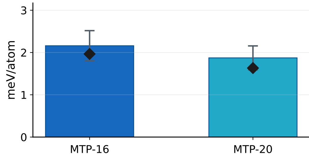
Energy MAE
