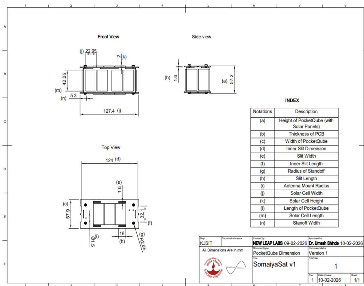
Fig. 2: Dimensions of SomaiyaSat (in mm)
