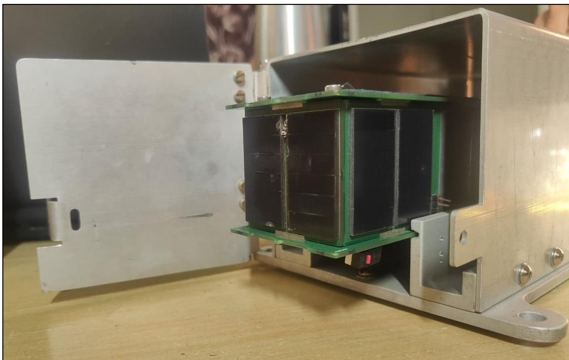
Fig. 1: SomaiyaSat and SomaiyaPOD
