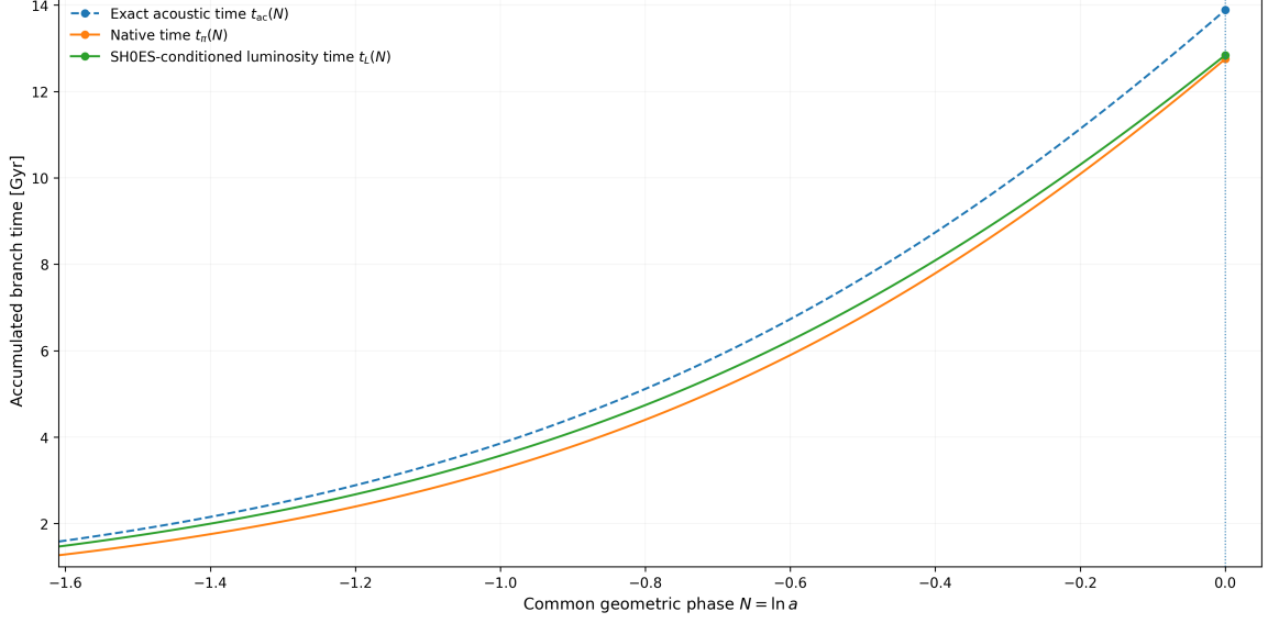
Figure 2: Common-phase branch-time trajectories over 0.20 \leq a \leq 1 . Every trajectory is evaluated against the same horizontal coordinate N_\pi = \ln a . The exact acoustic trajectory uses E_{ac} from Eq. (14); the native trajectory uses E_\pi ; and the luminosity trajectory uses the SH0ES-conditioned comparison realization of Eq. (51). The vertical dotted guide at N_\pi = 0 marks the present common phase. At that phase the integrated times are approximately t_\pi = 12.7541 Gyr, t_L = 12.8431 Gyr, and t_{ac} = 13.8852 Gyr.
