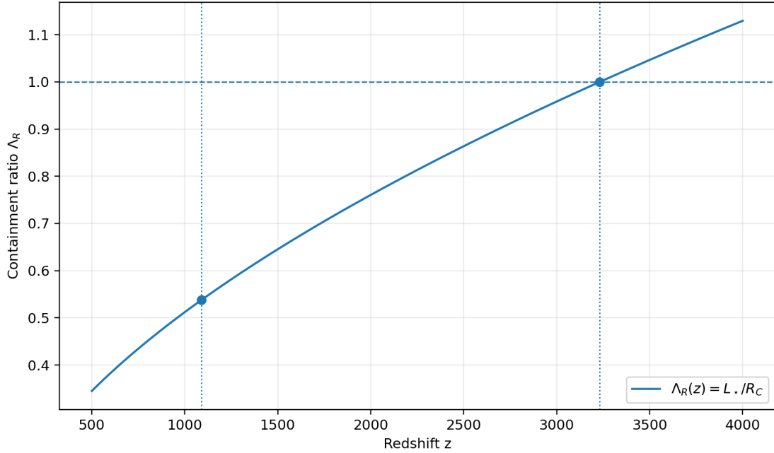
Figure 1: Native radial containment ratio \Lambda_R(z) = L_\star(z)/R_C(z) over the interval shown. The horizontal dashed line is the like-for-like containment boundary \Lambda_R = 1 . The trajectory crosses that boundary at z_{\text{enter}} = 3231.635355 , where L_\star = R_C = 4.292727257 Mpc. At the adopted Planck last-scattering phase z_\star = 1089.92 , the ratio has fallen to \Lambda_R = 0.53792156 , corresponding to L_\star = 12.72029287 Mpc inside R_C = 23.64711498 Mpc.
