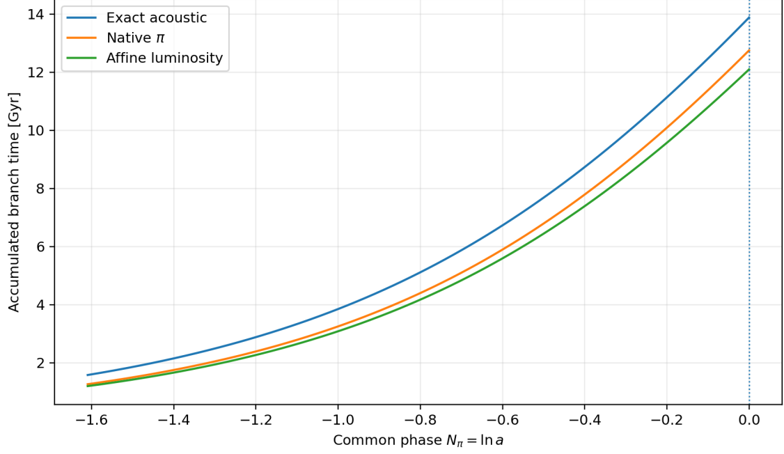
Figure 2: Common-phase branch-time trajectories over 0.20 \leq a \leq 1 . Every trajectory is evaluated against the same horizontal coordinate N_\pi = \ln a . The exact acoustic trajectory uses E_{ac} from Eq. (14); the native trajectory uses E_\pi ; and the luminosity trajectory uses the fixed affine clock map in Eq. (49). The vertical dotted guide at N_\pi = 0 marks the present common phase. At that phase the integrated times are approximately t_\pi = 12.7541 Gyr, t_L^{aff} = 12.0996 Gyr, and t_{ac} = 13.8852 Gyr.
