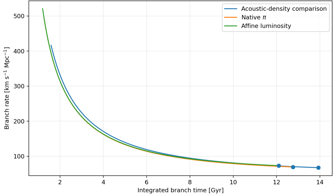
Figure 3: Late-time branch-rate trajectories over 0.20 \leq a \leq 1 . The native \pi branch, acoustic-density comparison, and fixed affine luminosity projection are evaluated on the same scale-factor sequence but each is plotted against its own integrated branch time t_b(a) . Horizontal alignment in this figure therefore does not denote equal geometric phase. The acoustic-density curve uses E_{ac,\rho} rather than the exact primordial acoustic projector E_{ac} , while the luminosity curve preserves the native shape with the fixed factor \Gamma_L^{aff} = \sqrt{10/9} . The endpoint labels 67.48, 69.42, and 73.1712 are the corresponding present rates in \text{km s}^{-1} \text{Mpc}^{-1} .
