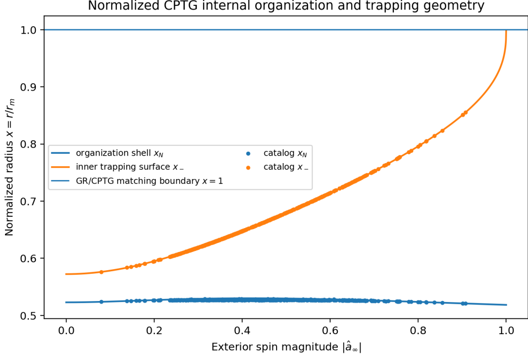
Figure 3: Normalized compact organization and trapping geometry. The Structural-Mode shell x_N remains inside the inner trapping surface x_- , while the GR/CPTG matching boundary is x = 1 . Points show the retained GWTC compact-component medians on the same registered curves.
