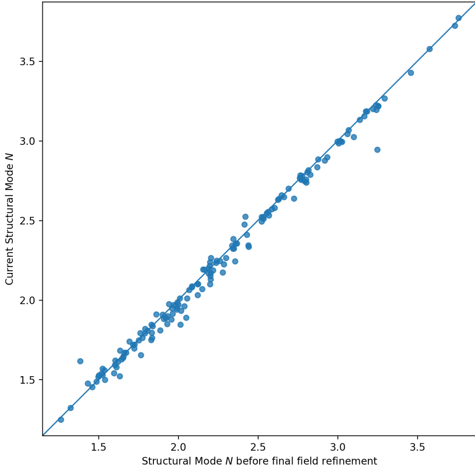
Figure 1: Galaxy Structural Mode before and after the final registered field refinement for the 153-galaxy primary sample. The diagonal denotes equality. The close object-by-object agreement, r = 0.995854 , shows that the refinement materially improves the gravitational solution without radically reorganizing the downstream Structural Mode coordinate. Twenty-eight galaxies cross a current named CSMI interval boundary; the continuous N values remain the primary structural measurements.
