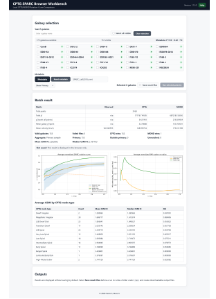
Figure 2: CPTG SPARC Browser Workbench v1.13.0 in batch-analysis mode.
