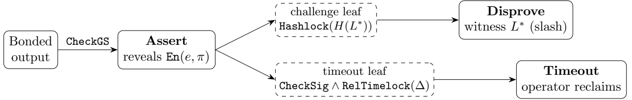
Figure 1: The Assert output carries two tapleaves; the verdict decides which is spendable. A false verdict lets a challenger open the hashlock ( Disprove , slash); otherwise the timelock lets the operator reclaim the bond ( Timeout ).
