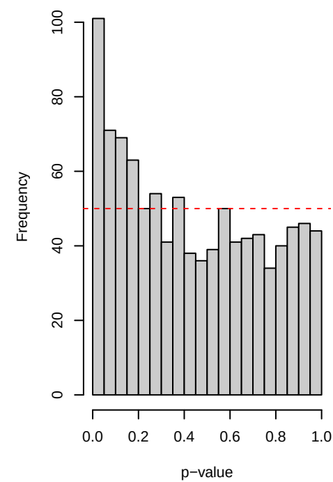
Reproducibility – bca
