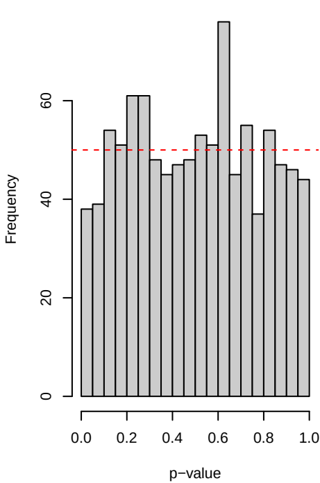
Repeatability – recentred
