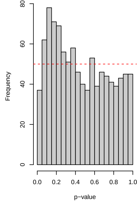
Reproducibility – basic
