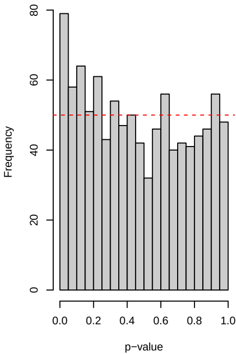
Reproducibility – recentred
