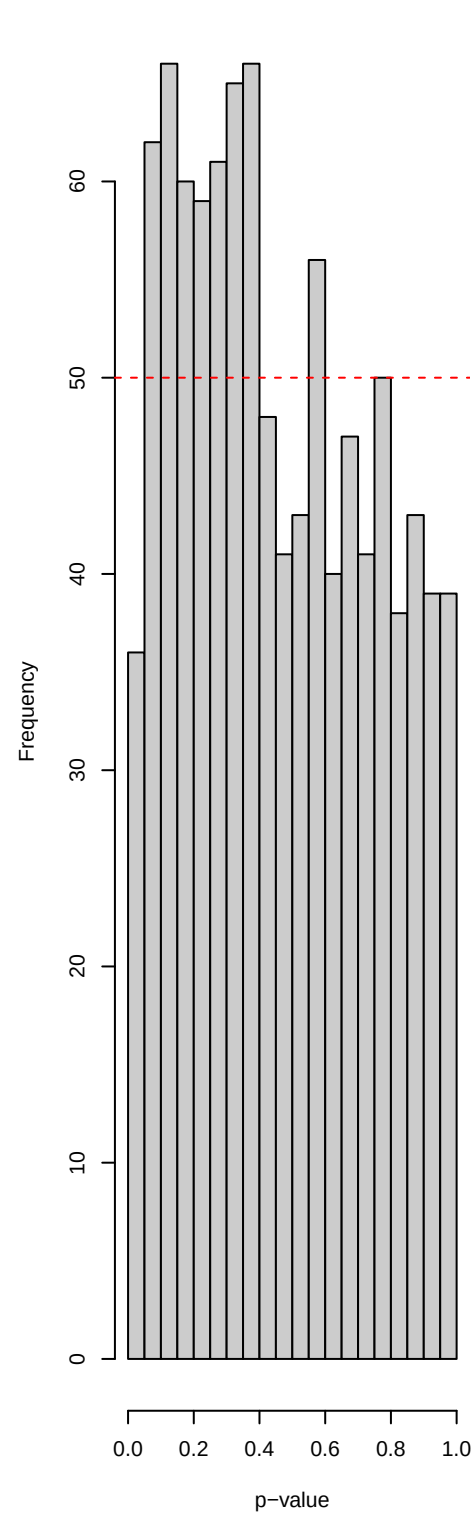
Reproducibility – basic
