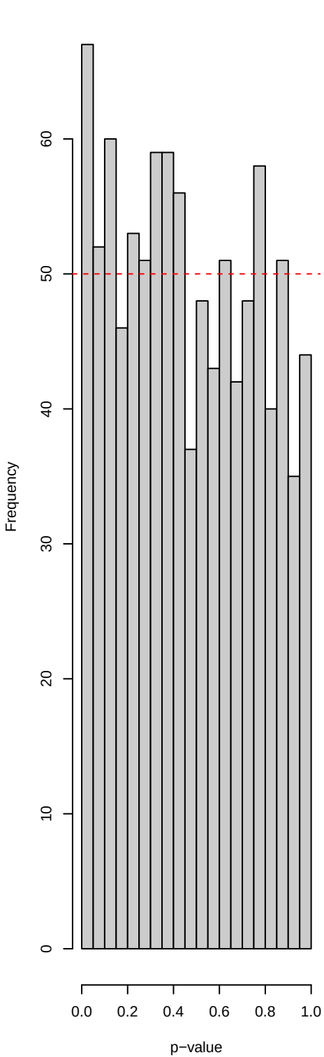
Reproducibility – recentred
