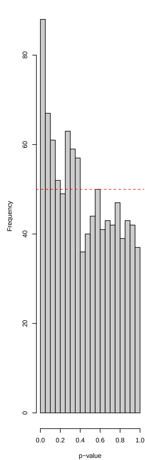
Reproducibility – bca
