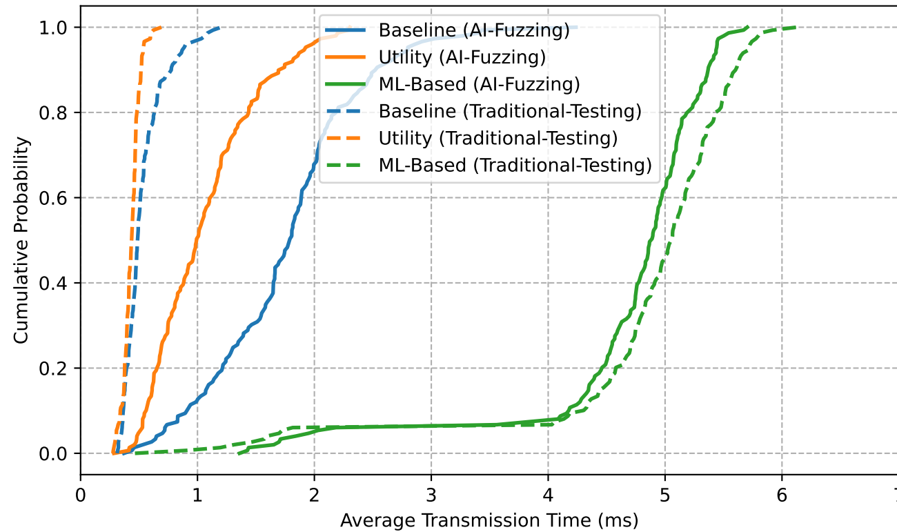
CDF of Average Transmission Time (ms) AI Fuzzing vs Traditional Testing - Stable Mobility
