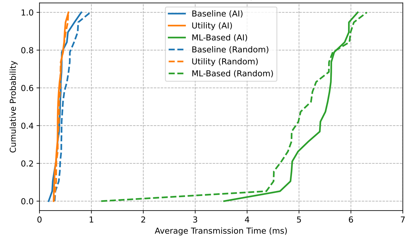
CDF of Average Transmission Time (ms) Scenario: Stable High Load
