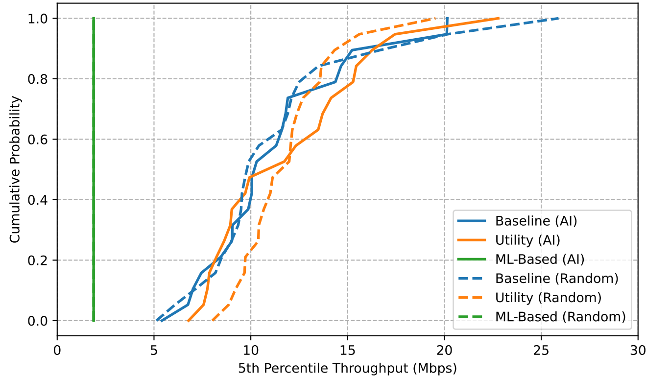
CDF of 5th Percentile Throughput (Mbps) Scenario: Stable Mobility
