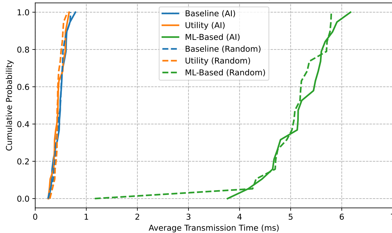
CDF of Average Transmission Time (ms) Scenario: Stable Mobility
