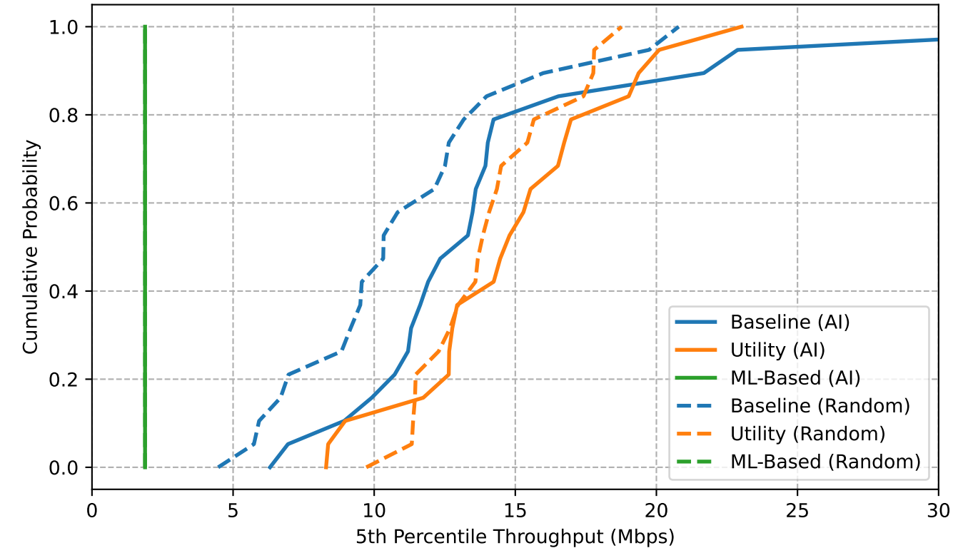
CDF of 5th Percentile Throughput (Mbps) Scenario: Stable High Load
