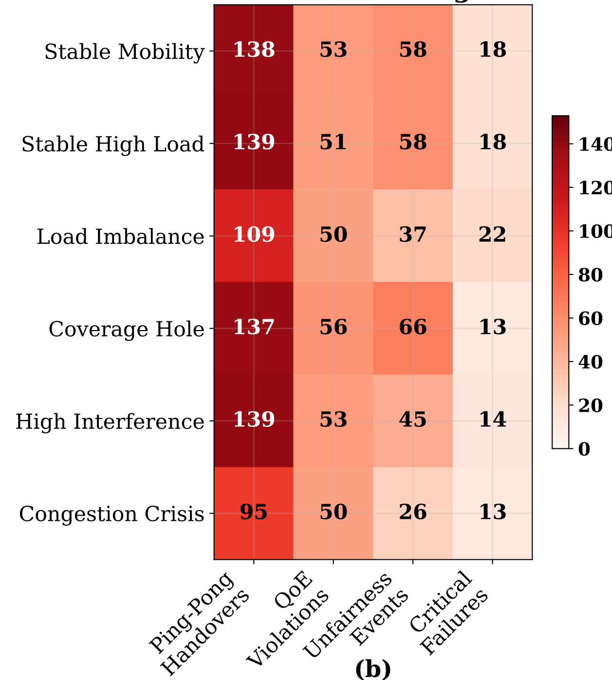
Hill Climbing
