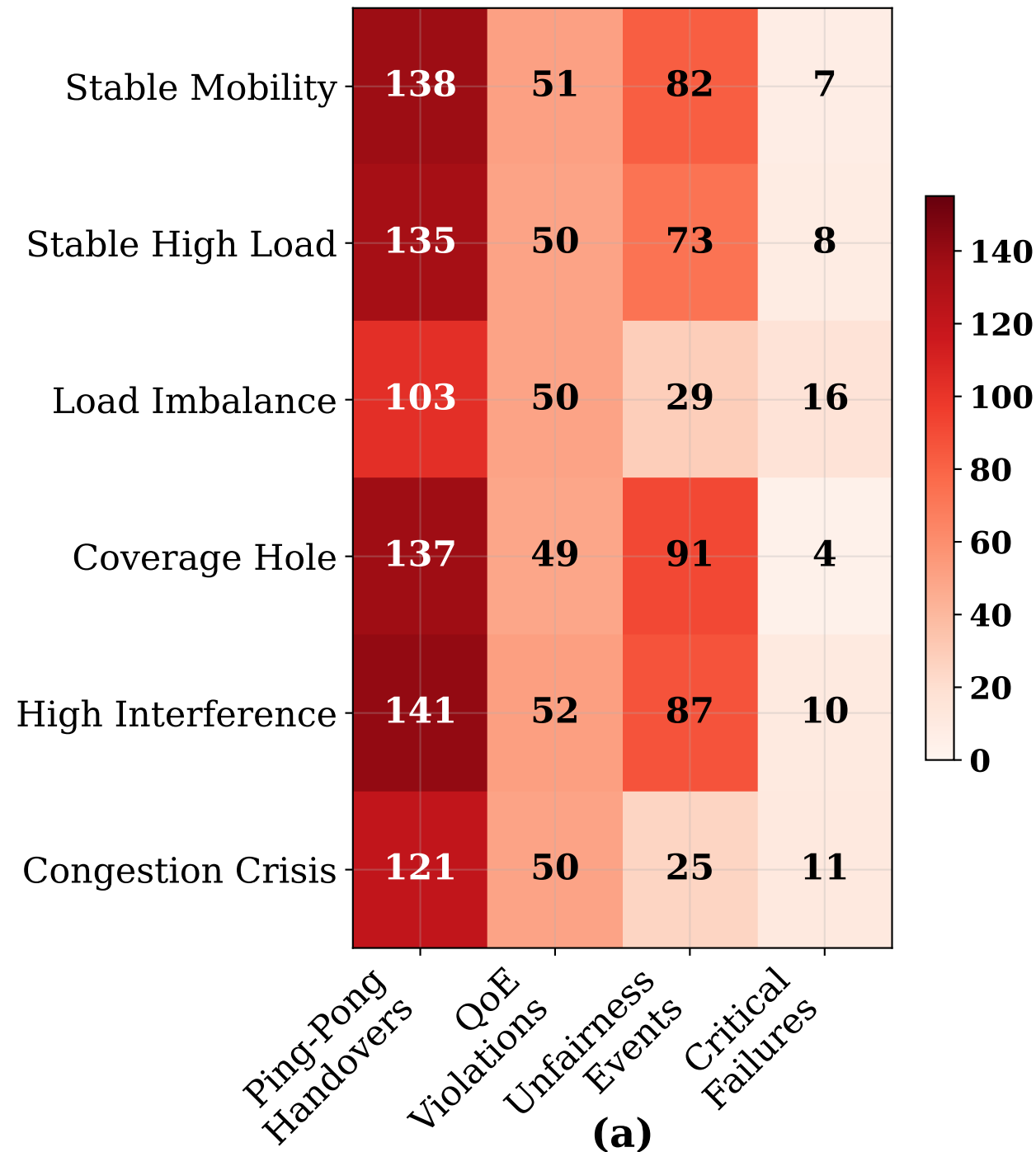
Random
