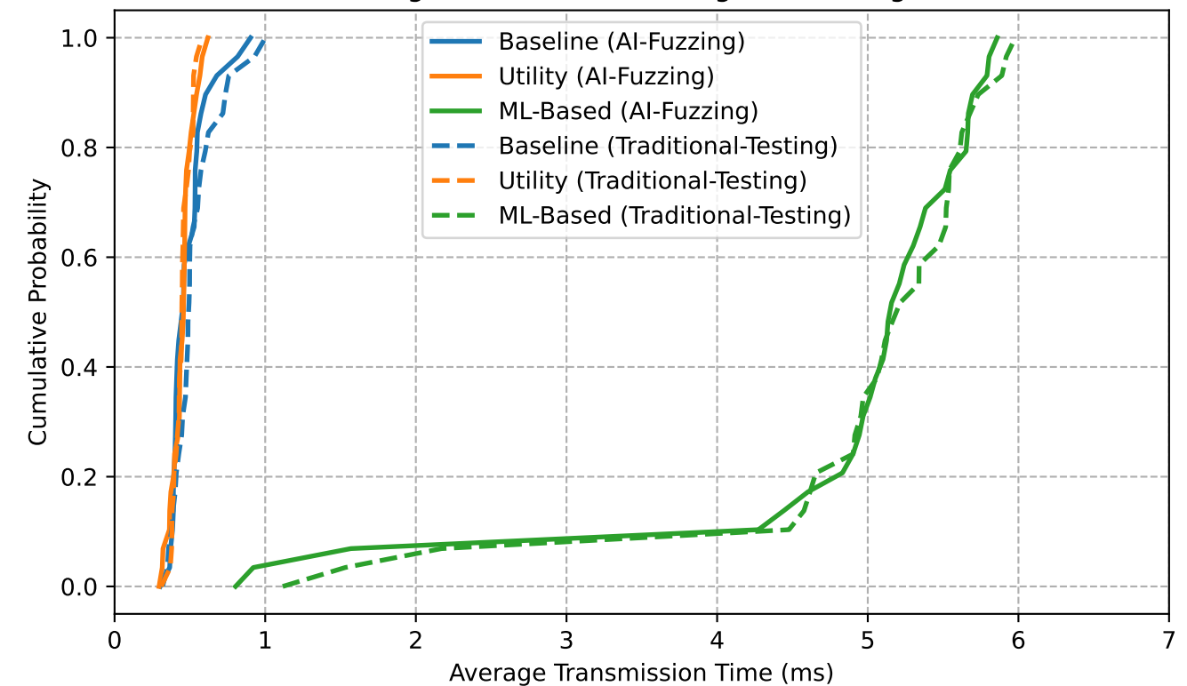
CDF of Average Transmission Time (ms) AI Fuzzing vs Traditional Testing - Stable High Load
