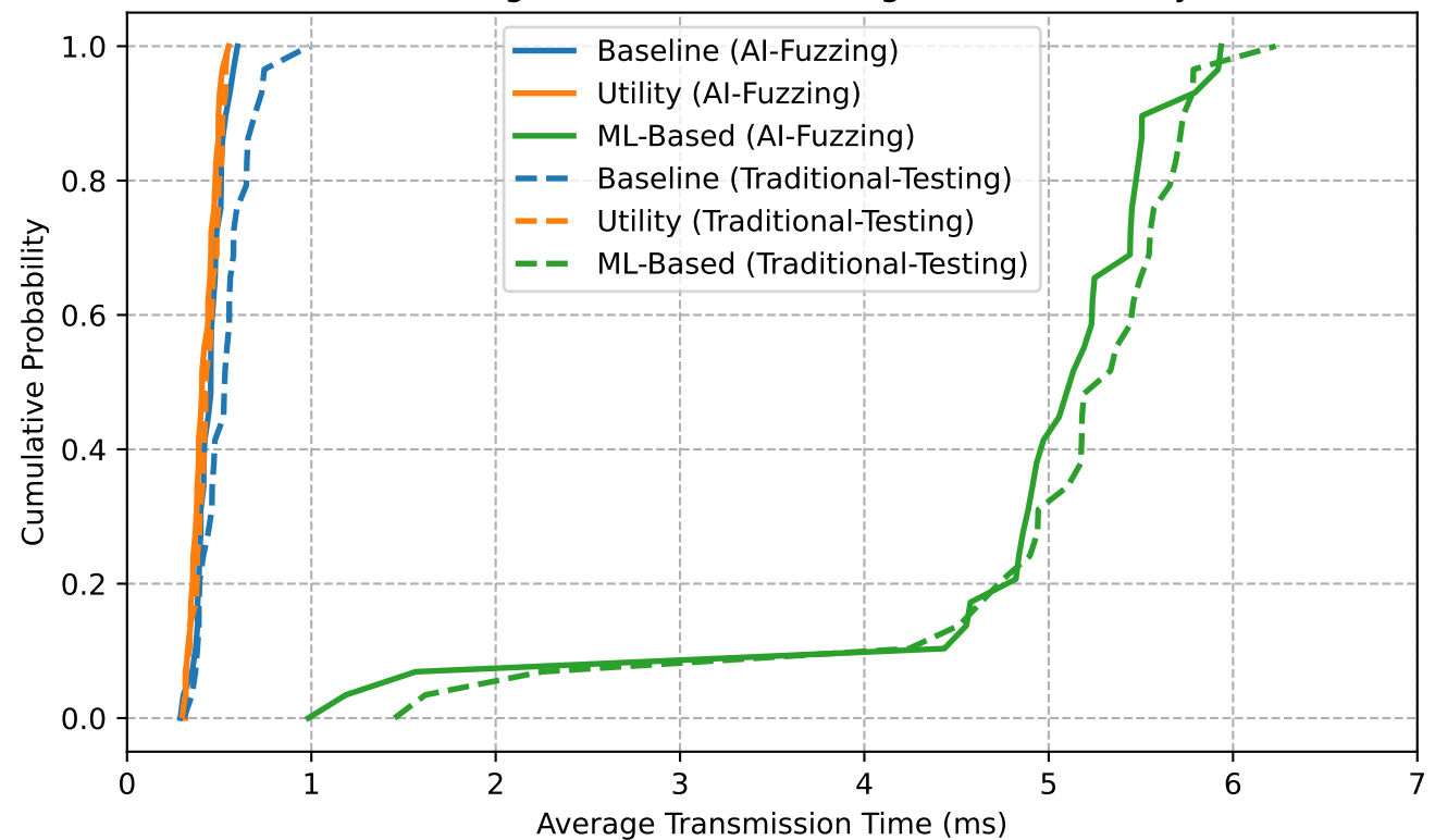
CDF of Average Transmission Time (ms) AI Fuzzing vs Traditional Testing - Stable Mobility
