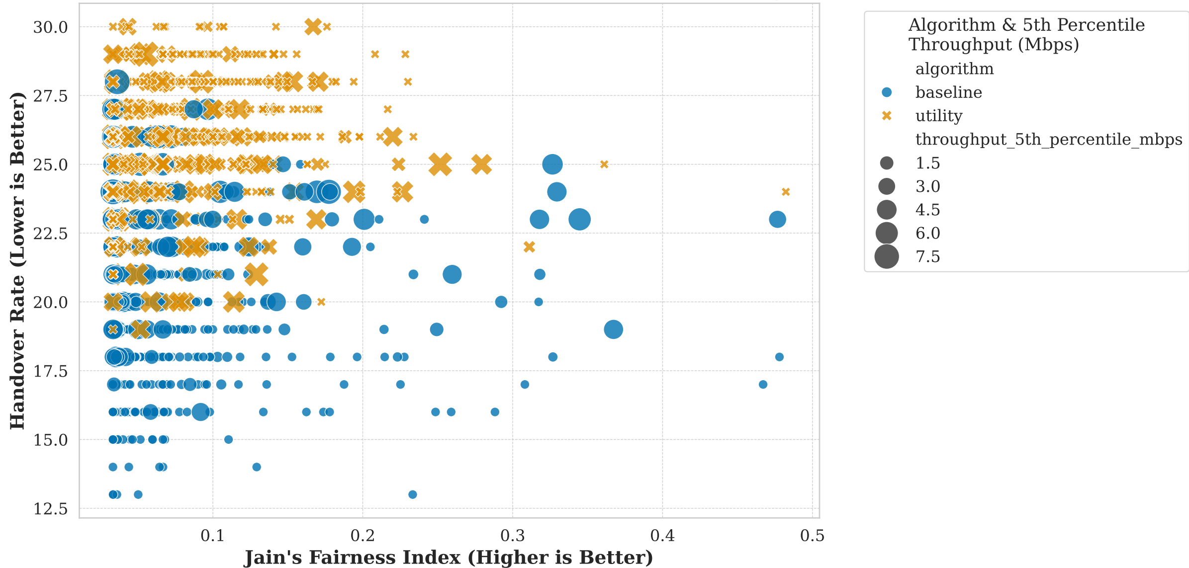
QoE Trade-off: Fairness vs. Handovers vs. Worst-User Throughput
