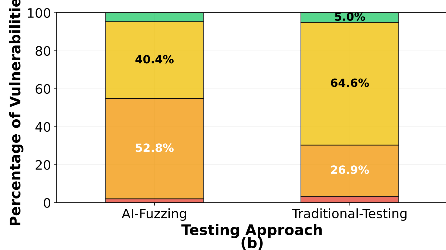
Normalized Severity Distribution (%)
