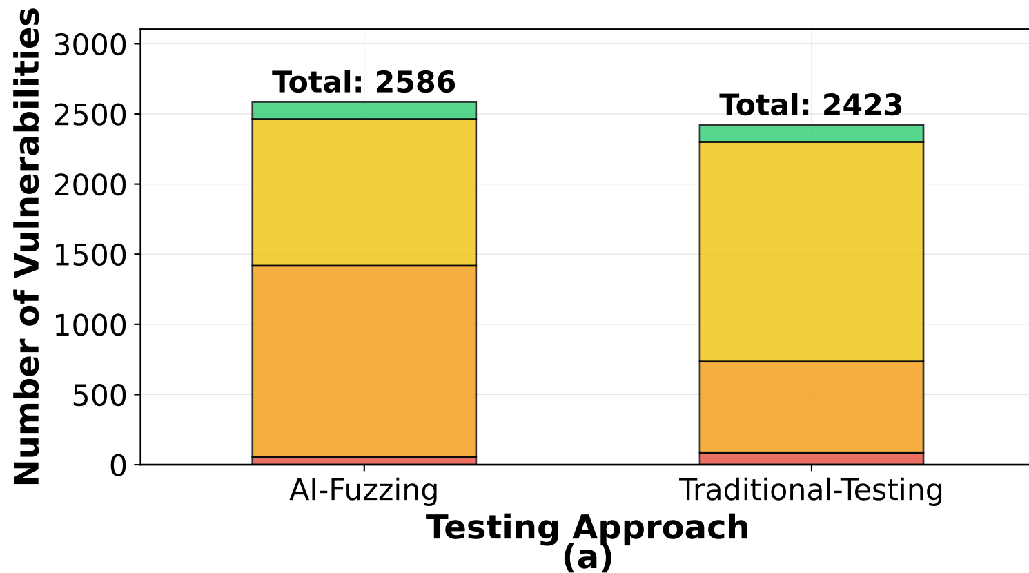
Absolute Vulnerability Counts by Severity
