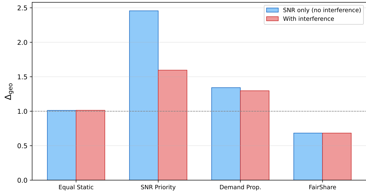
Impact of Interference on Geographic Disparity — Kuiper Shell 1
