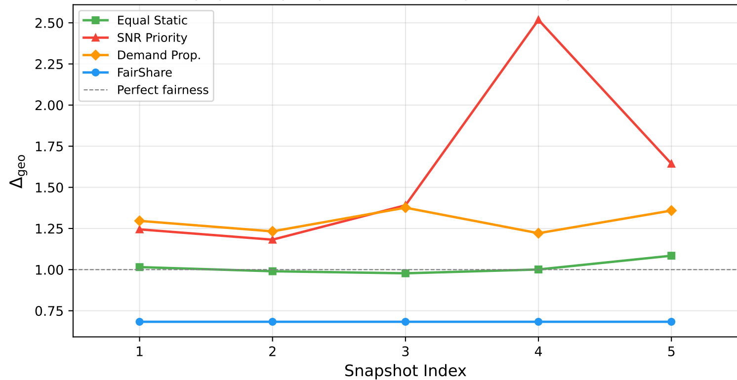
Geographic Disparity Over Orbital Snapshots — Kuiper Shell 1
