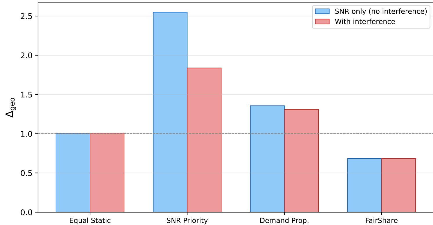
Impact of Interference on Geographic Disparity — Starlink Shell 1
