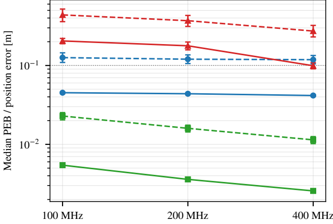
Fig. 2. Median single-epoch position error bound (LoS-only, map-aided) and median estimator error versus bandwidth, for epochs with LoS to both O-RUs and with a blocked O-RU; main configuration (95% CI). The bound and the error are different quantities (Section IV).
