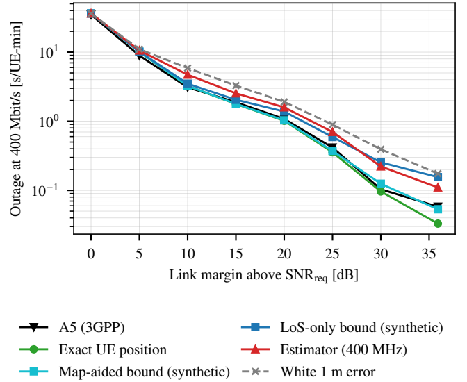
Fig. 3. Outage at 400 Mbit/s versus link margin. Except for A5, every curve is the blockage-aware planner with perfect blocker tracks, fed with the indicated UE position (bound-level errors are synthetic).
