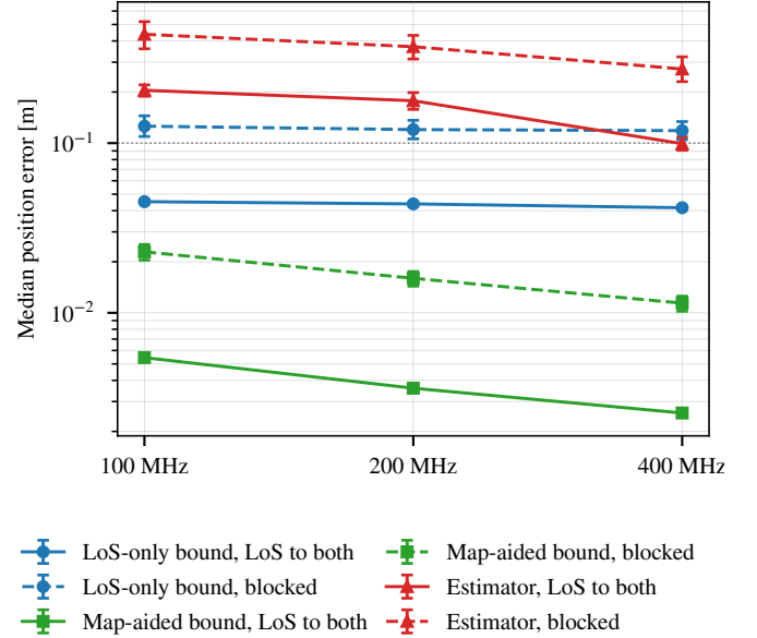
Fig. 1. Median single-epoch position error bound (LoS-only, map-aided) and median estimator error versus bandwidth, for epochs with LoS to both O-RUs and with a blocked O-RU; main configuration (95% CI). The bound and the error are different quantities (Section IV).
