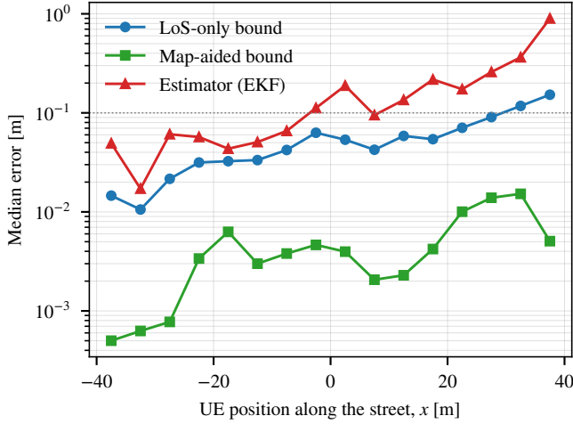
Fig. 2. Median bound and estimator error along the sidewalk (5-m bins of the UE position); main configuration.
