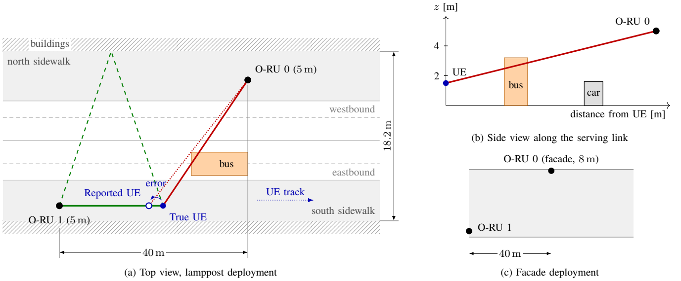
Fig. 1. Scenario (to scale). (a) Two neighboring cells share the street; O-RU 1 is 40 m further along the street than O-RU 0. The true serving link (solid red) crosses the bus, whereas the link predicted from the reported UE position (dotted) passes it, so a position error turns into a missed blockage prediction; green: link to the other cell and one of its facade reflections (dashed). (b) The LoS passes through a bus but above a car. (c) In the facade deployment, O-RU 0 is mounted on the north facade at 8 m.
