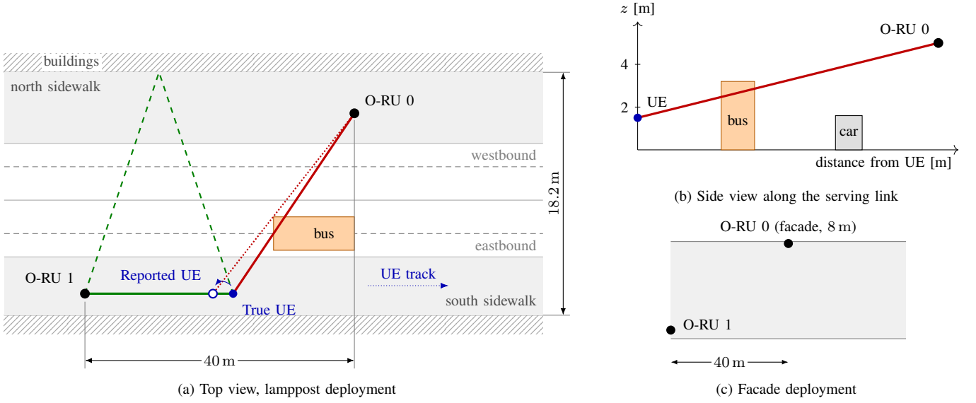
Fig. 1. Scenario (to scale). (a) Two neighboring cells share the street; O-RU 0 and O-RU 1 are on 5 m lampposts, 40 m apart along the street. The true serving link (solid red) crosses the bus, whereas the link predicted from the reported UE position (dotted) passes it, so a position error turns into a missed blockage prediction; green: link to the other cell and one of its facade reflections (dashed). (b) The LoS passes through a bus but above a car. (c) In the facade deployment, O-RU 0 is mounted on the north facade at 8 m.
