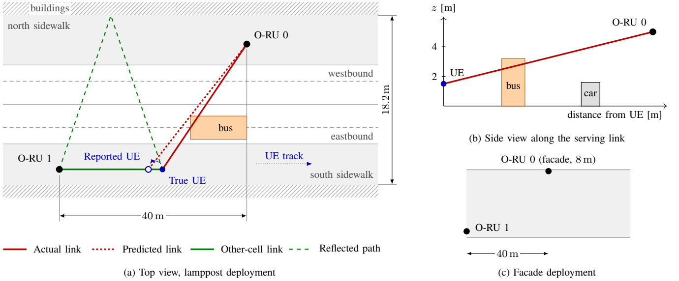
Fig. 1. Scenario geometry (dimensions indicated; axes scaled independently). (a) Two neighboring cells share the street; O-RU 0 and O-RU 1 are on 5 m lampposts, 40 m apart along the street. The true serving link (solid red) crosses the bus, whereas the link predicted from the reported UE position (dotted) passes it, so a position error turns into a missed blockage prediction; green: link to the other cell and one of its facade reflections (dashed). (b) The LoS passes through a bus but above a car. (c) In the facade deployment, O-RU 0 is mounted on the north facade at 8 m.
