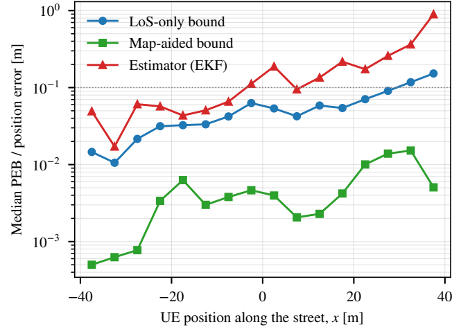
Fig. 3. Median bound and estimator error along the sidewalk (5-m bins of the UE position); main configuration.
