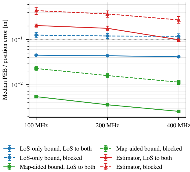
Fig. 2. Median single-epoch position error bound (LoS-only, map-aided) and median estimator error versus bandwidth, for epochs with LoS to both O-RUs and with a blocked O-RU; main configuration (95% CI). The bound and the error are different quantities (Section IV).
