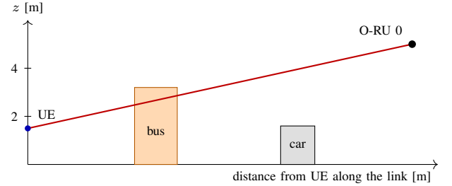
(b) Side view along the serving link
