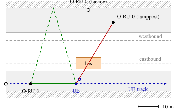
(a) Top view of the periodic street section
