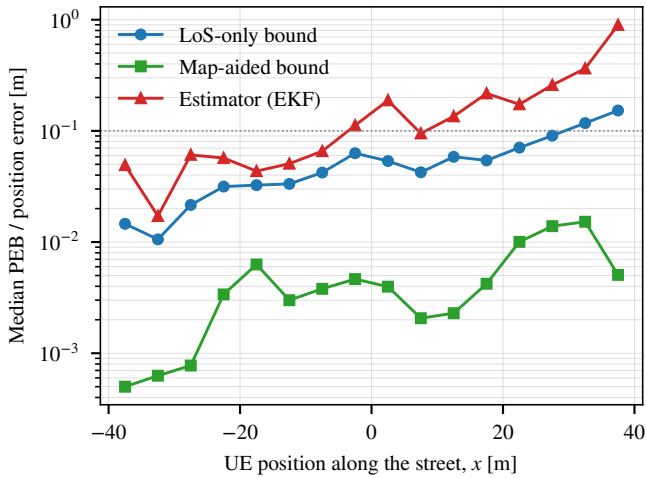
Fig. 3. Median bound and estimator error along the sidewalk (5-m bins of the UE position); main configuration.
