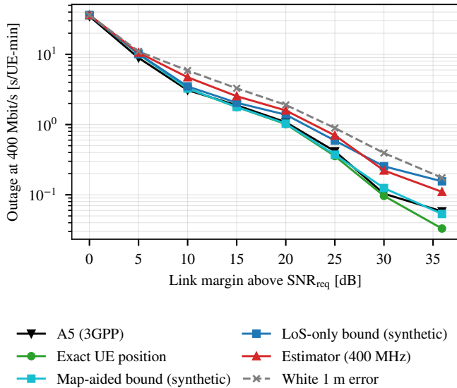
Fig. 4. Outage at 400 Mbit/s versus link margin. Except for A5, every curve is the blockage-aware planner with perfect blocker tracks, fed with the indicated UE position (bound-level errors are synthetic).
