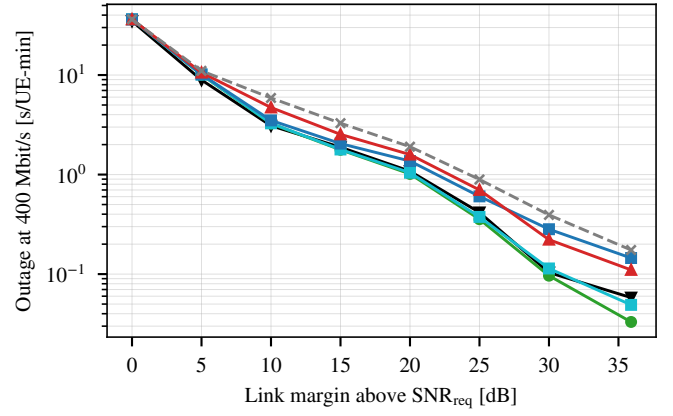
Fig. 3. Outage at 400 Mbit/s versus link margin: 3GPP A5 and the blockage-aware planner with perfect blocker tracks, fed with UE positions of different quality (bound-level errors are synthetic).
