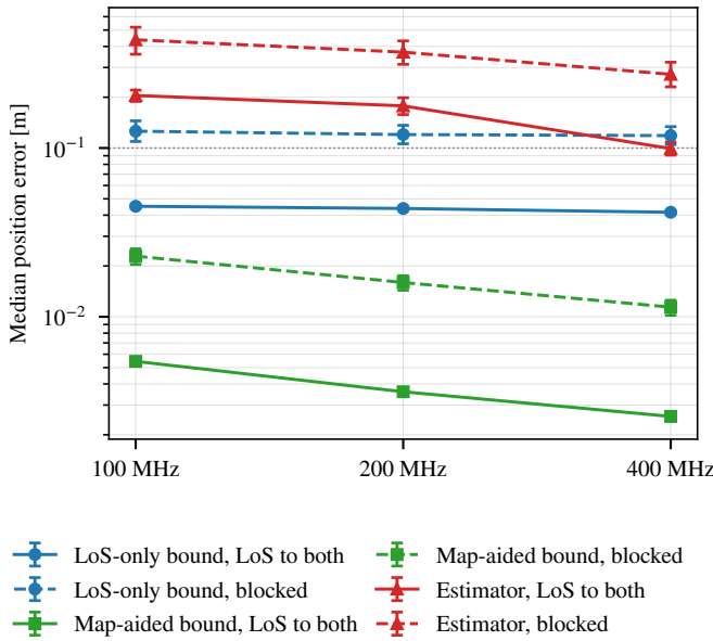
Fig. 1. Median single-epoch position error bound (LoS-only, map-aided) and median estimator error versus bandwidth, for epochs with LoS to both O-RUs and with a blocked O-RU; main configuration (95% CI). The bound and the error are different quantities (Section IV).
