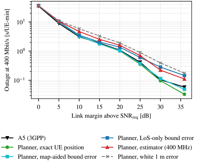
Fig. 4. Outage at 400 Mbit/s versus link margin: 3GPP A5 and the blockage-aware planner with perfect blocker tracks, fed with UE positions of different quality (bound-level errors are synthetic).
