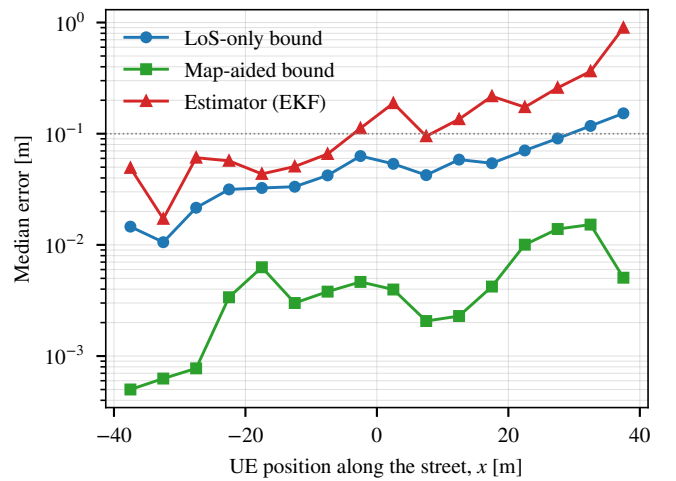
Fig. 2. Median bound and estimator error along the sidewalk (5-m bins of the UE position); main configuration.
