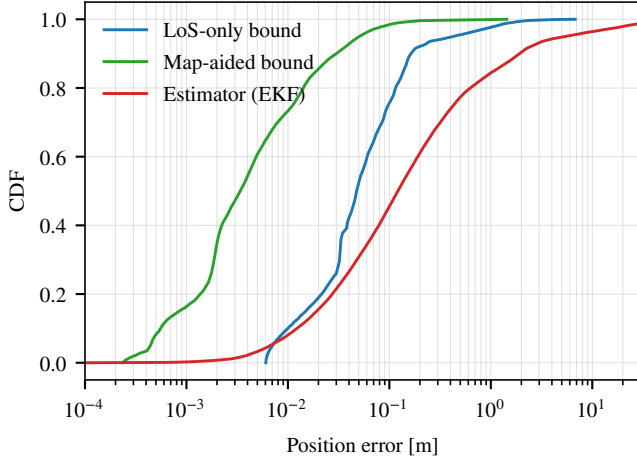
Fig. 3. Distributions over all epochs of the LoS-only and map-aided PEB (i.e., of the geometry) and of the estimator error (main configuration). The curves describe different quantities and are shown for scale only.
