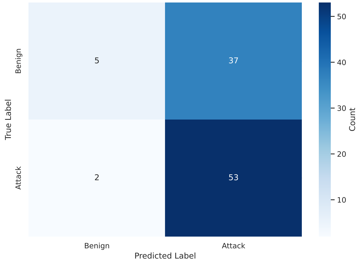
Confusion Matrix
