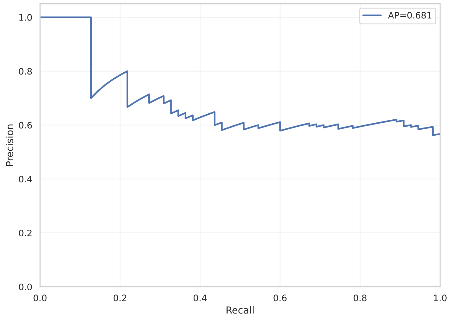
Precision-Recall Curve
