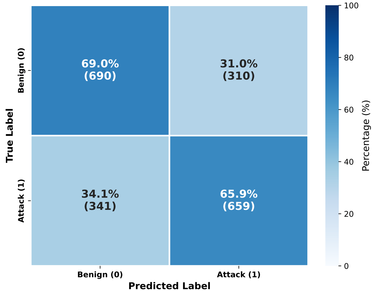
Scenario A: Single-hop Downlink
