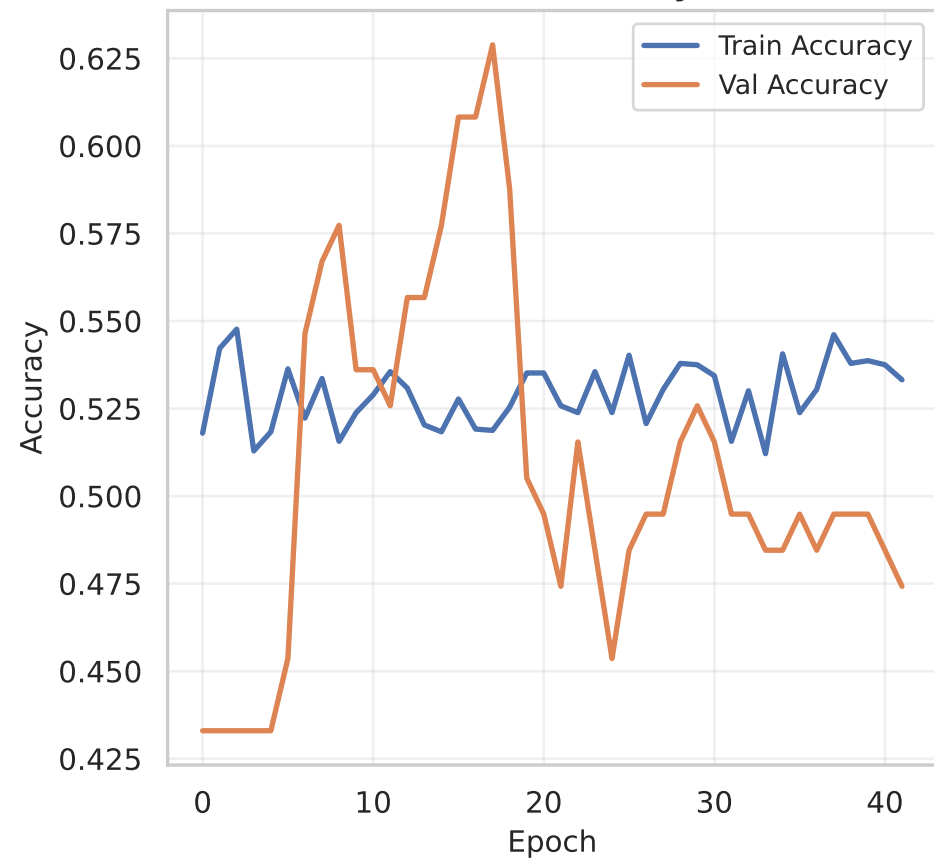
Model Accuracy
