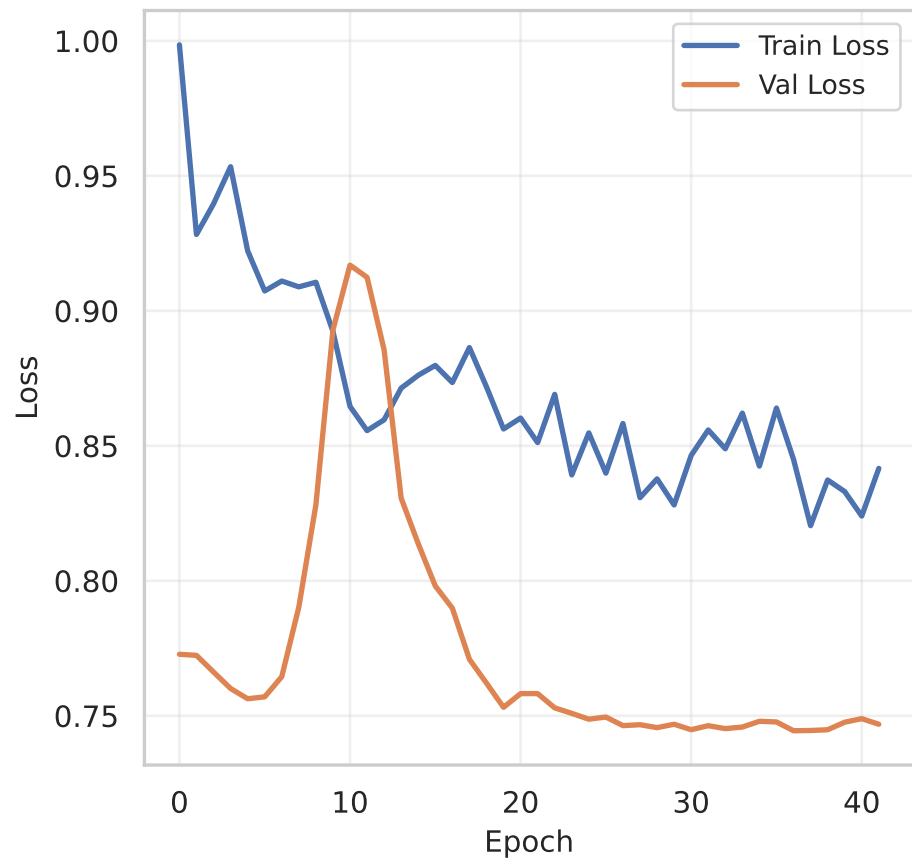
Model Loss
