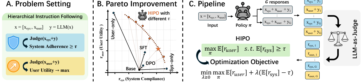
Figure 1: The HIPO framework for hierarchical instruction following. (A) Problem formulation: maximizing user utility ( \mathbb{E}[r_{\text{user}}] ) subject to a system adherence constraint ( \mathbb{E}[r_{\text{sys}}] \geq \tau ). (B) Performance illustration: HIPO improves the trade-off between system compliance and user utility relative to baselines. (C) The optimization pipeline: distinct system ( r_{\text{sys}} ) and user ( r_{\text{user}} ) rewards are derived for constrained optimization.
