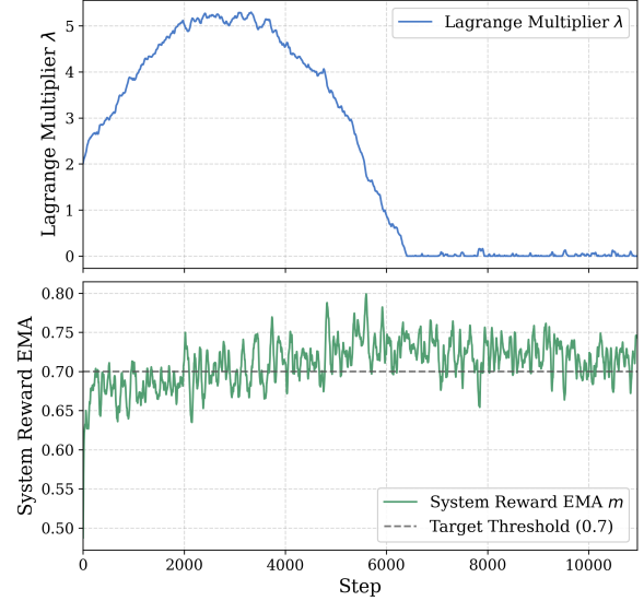
Figure 3: Training dynamics of the Lagrange multiplier \lambda (top) and the system reward EMA (bottom). The multiplier increases to penalize the model when the reward is below the 0.7 target threshold, and automatically drops to zero once the constraint is consistently satisfied.
