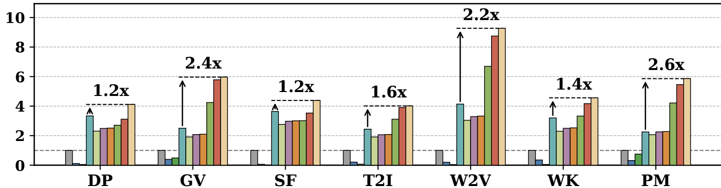
Normalized QPS/W
