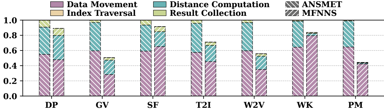
Normalized Latency
