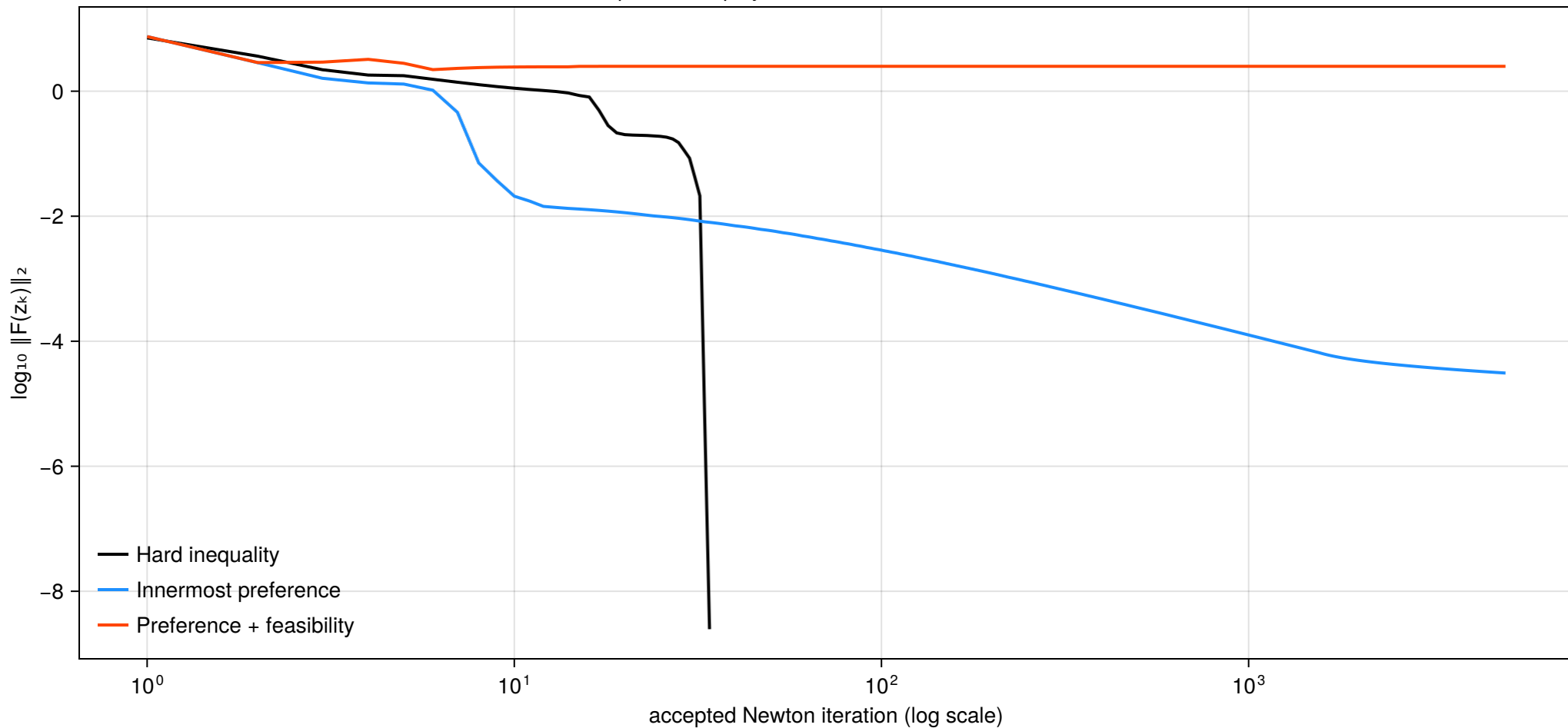
Explicit three-player solve: KKT residual histories
