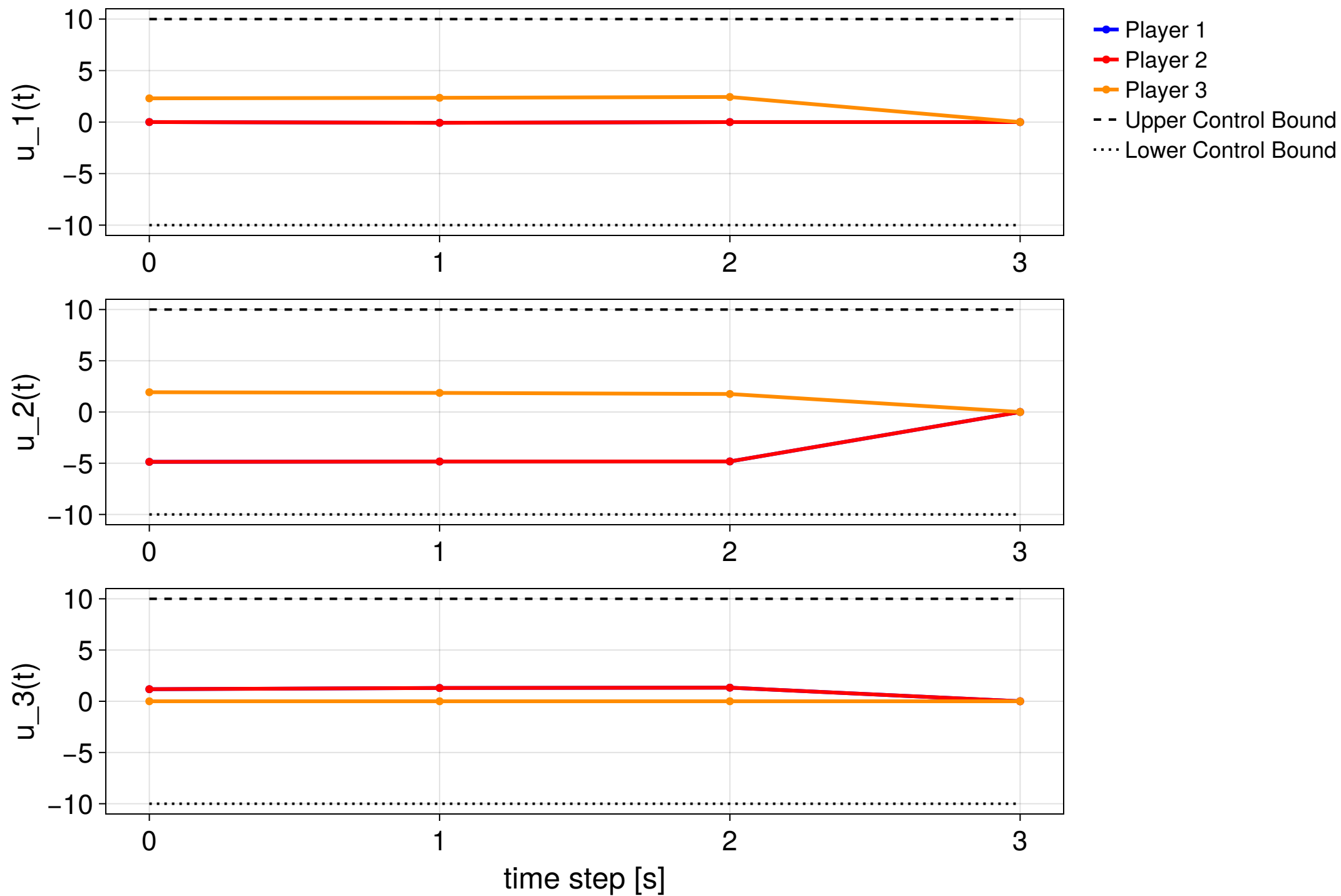
MPC step 3/3
