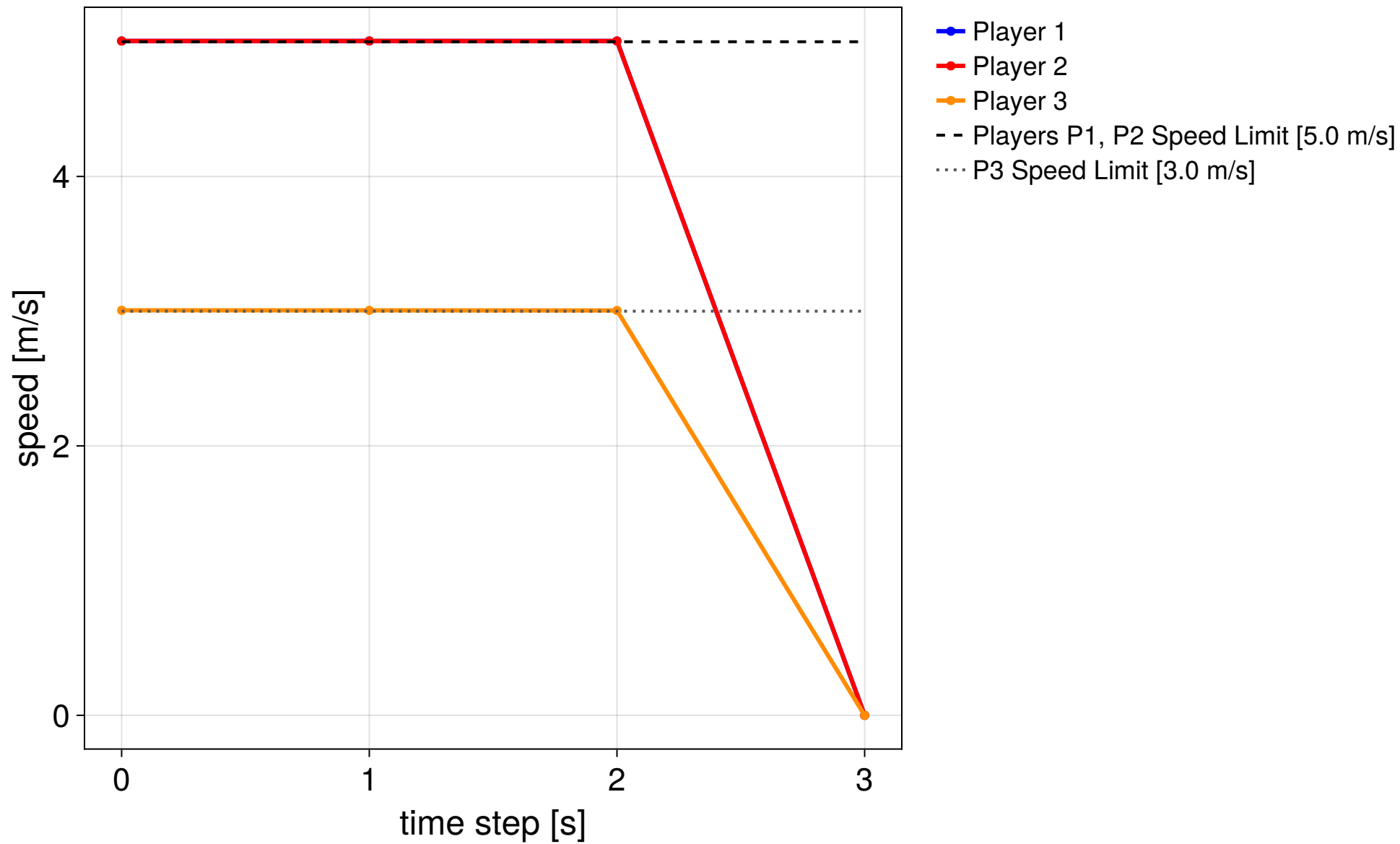
MPC step 1/3
