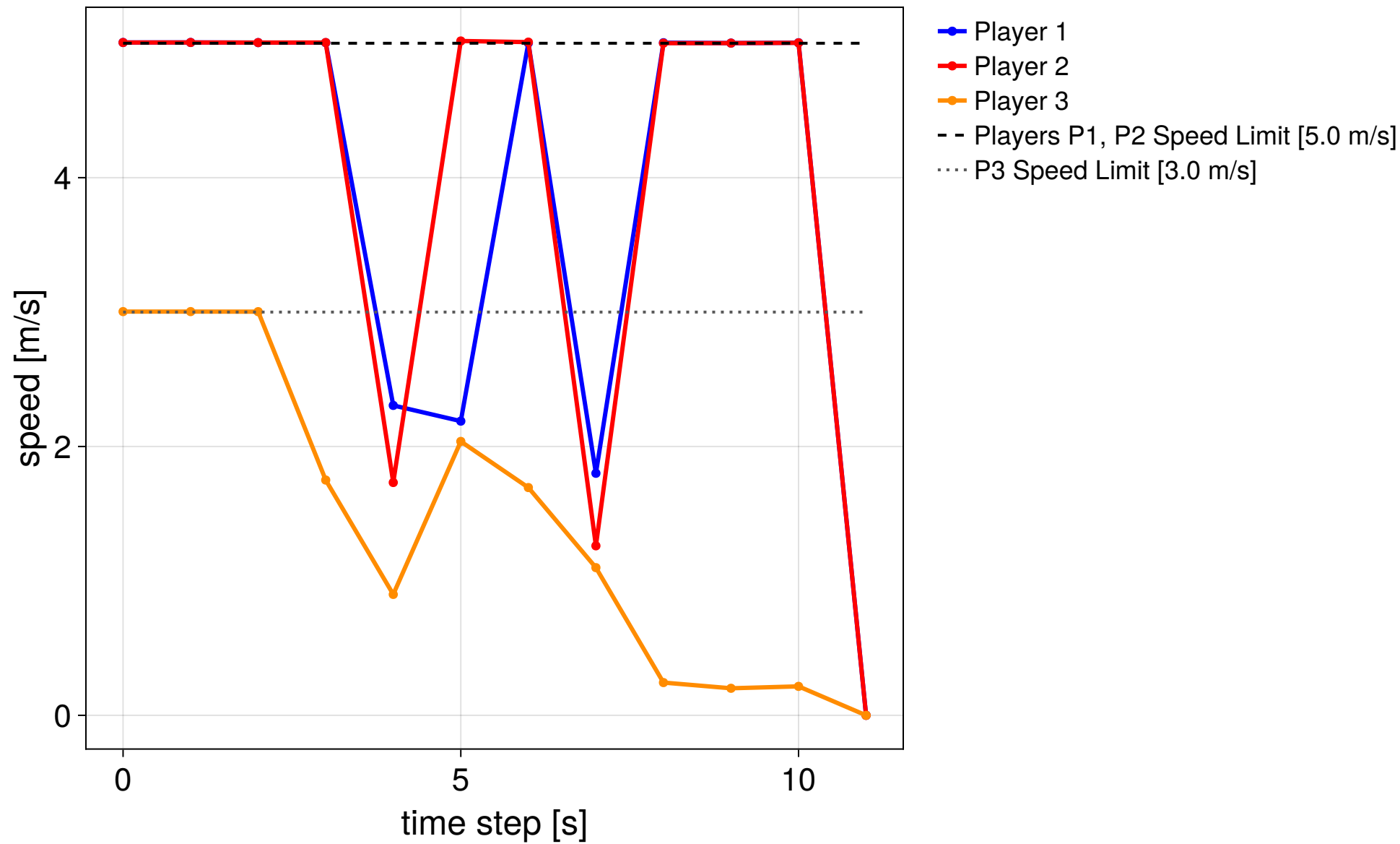
MPC step 29/30 — NOT CONVERGED (KKT error 0.792)
