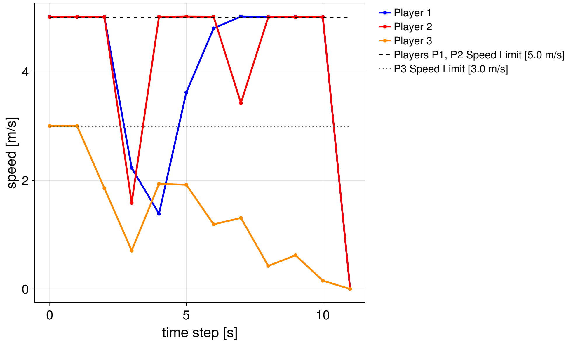
MPC step 30/30 — NOT CONVERGED (KKT error 0.835)
