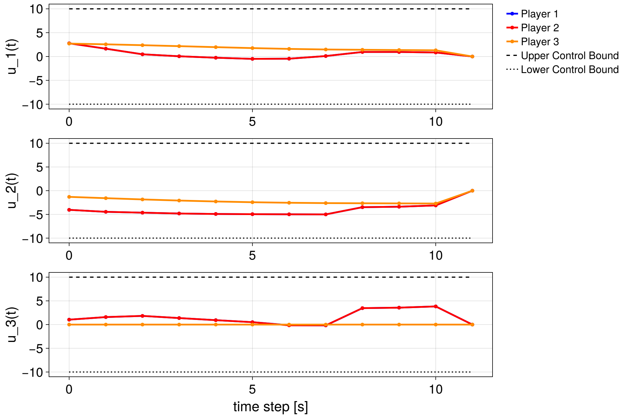
MPC step 12/20
