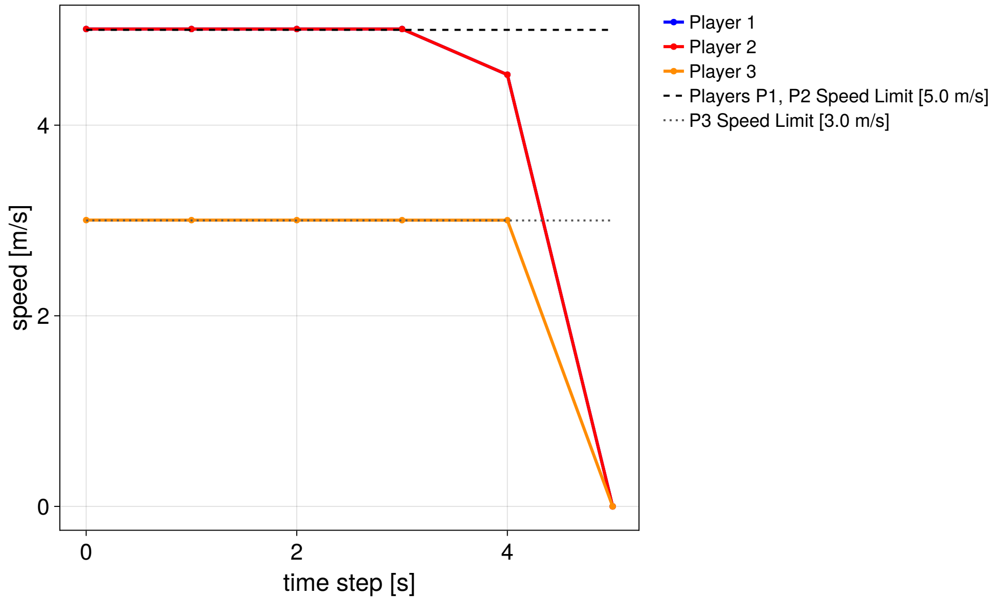
MPC step 19/30
