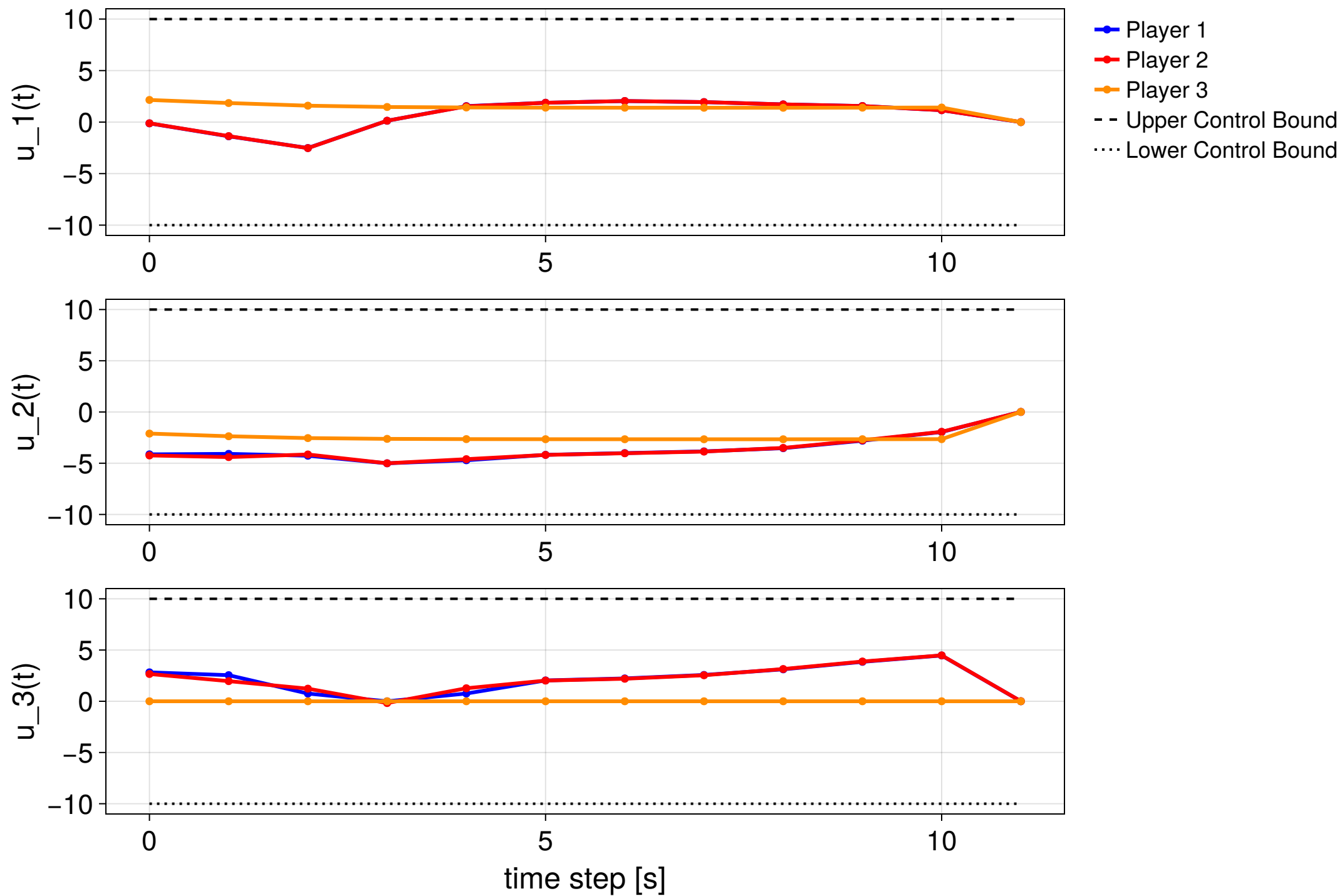
MPC step 13/15 — NOT CONVERGED (KKT error 1.29)
