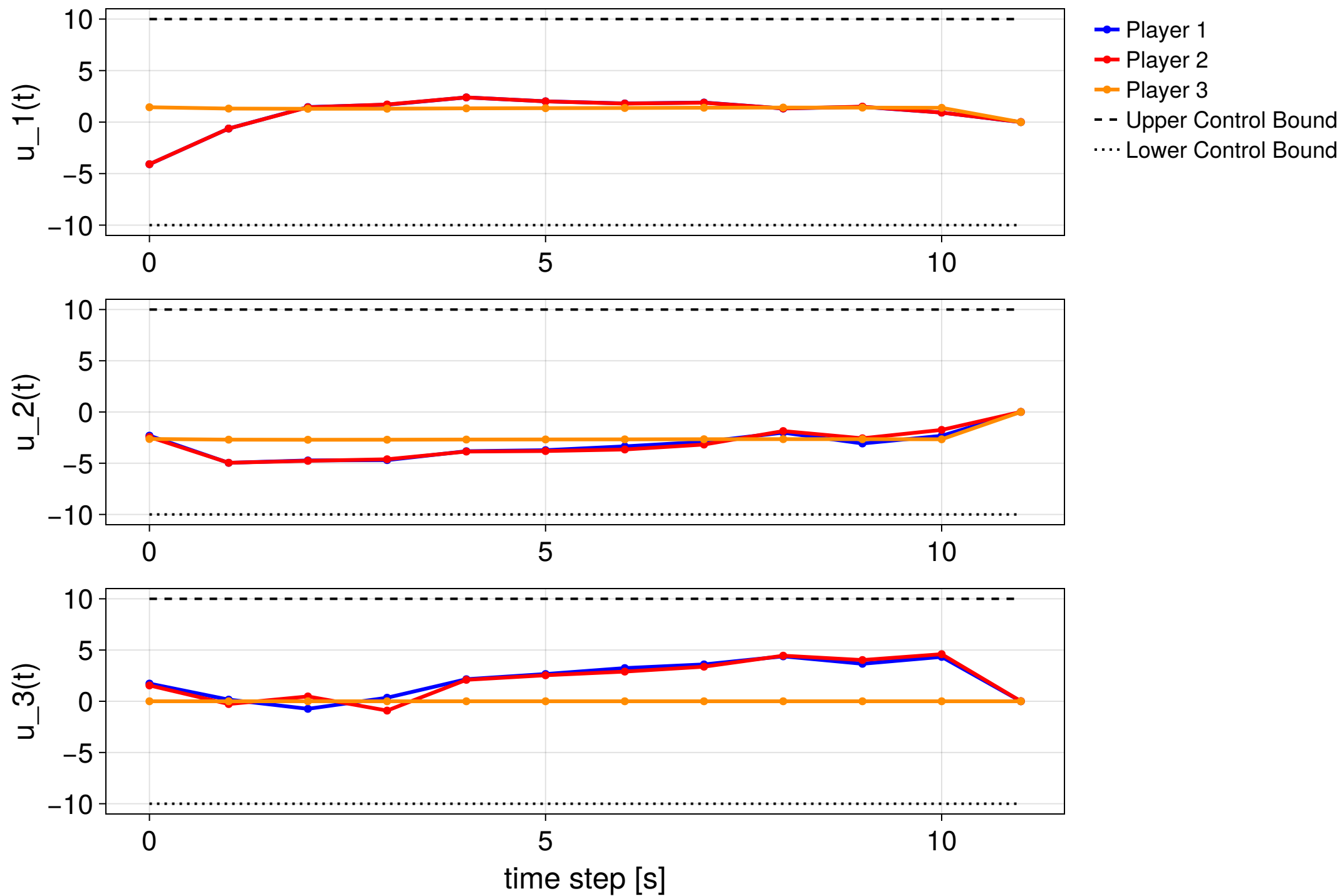
MPC step 15/15 — NOT CONVERGED (KKT error 0.154)
