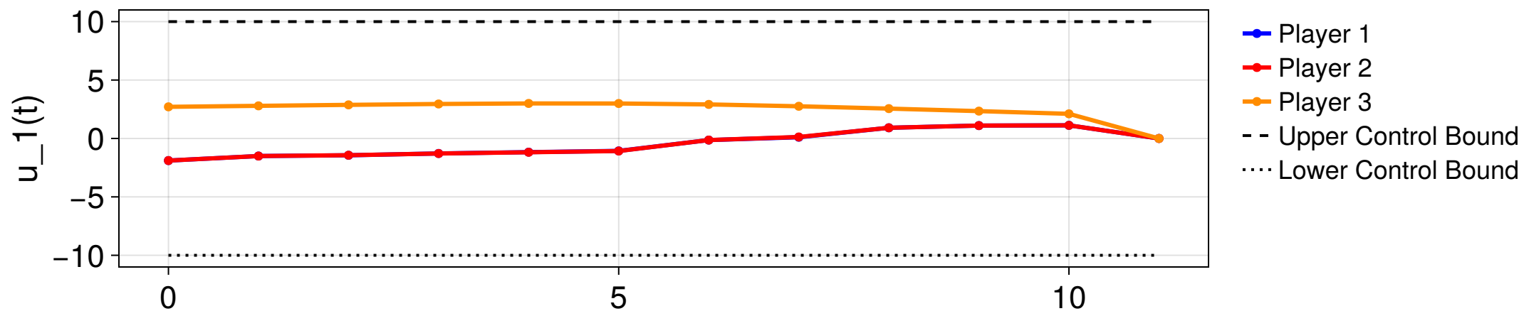
MPC step 6/15 — NOT CONVERGED (KKT error 0.427)
