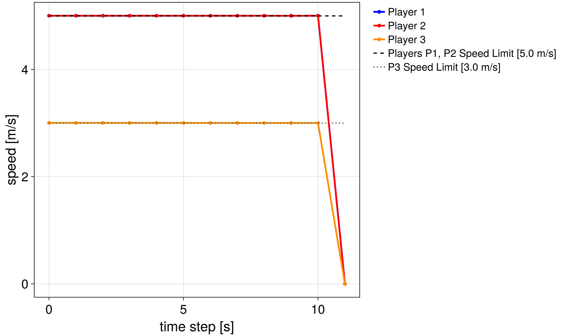
MPC step 5/15 — NOT CONVERGED (KKT error 0.0318)
