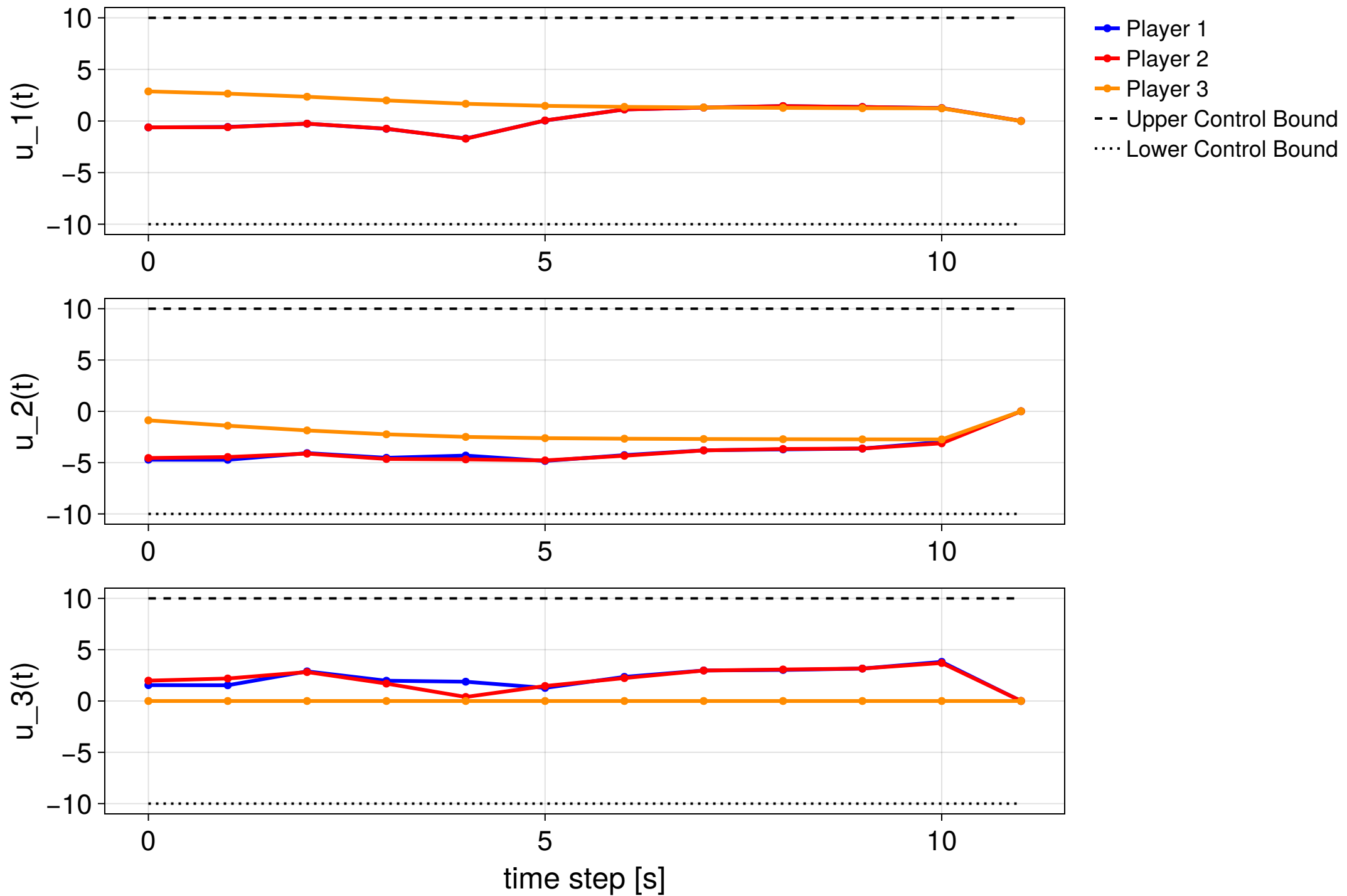
MPC step 11/25 — NOT CONVERGED (KKT error 0.0613)
