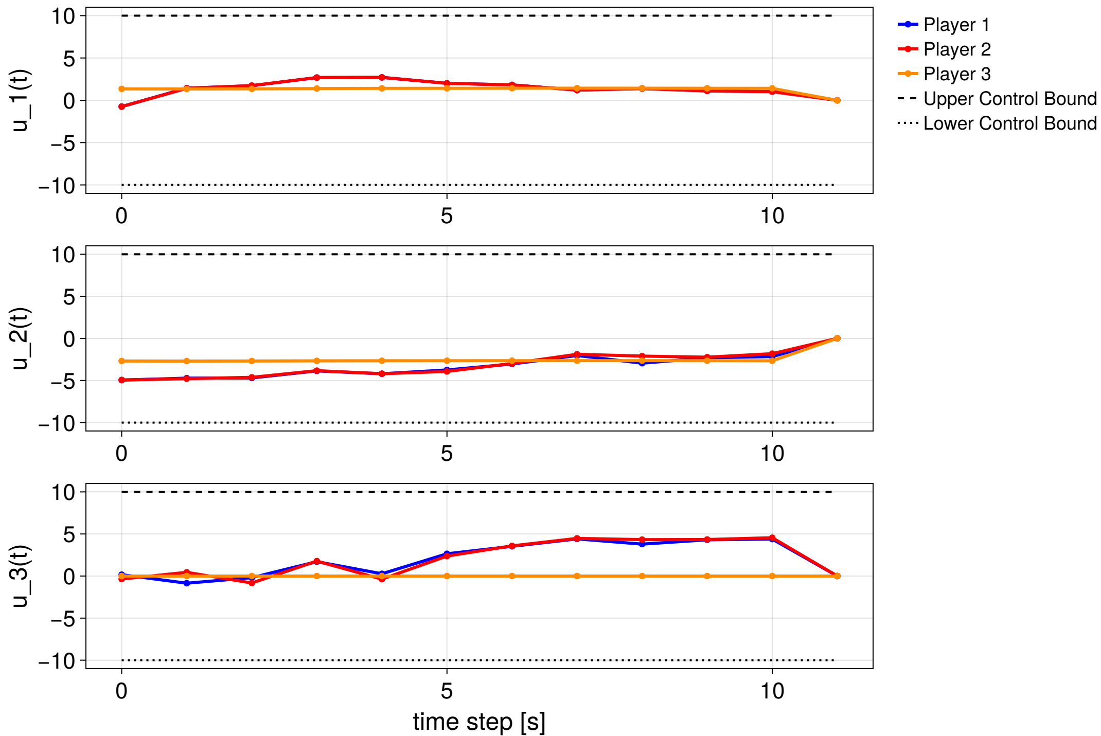
MPC step 16/25 — NOT CONVERGED (KKT error 0.442)
