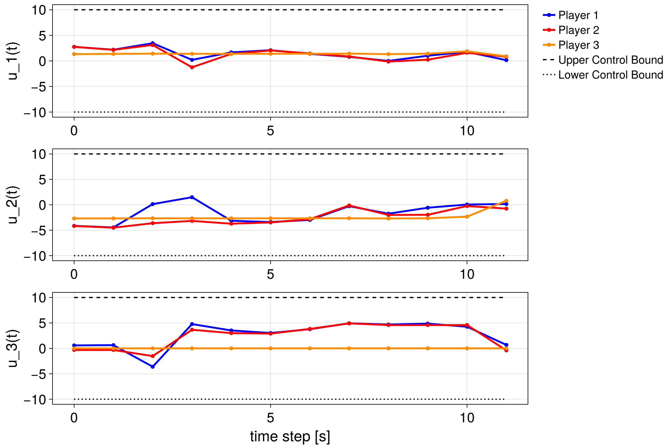
MPC step 20/25 — NOT CONVERGED (KKT error 0.0792)
