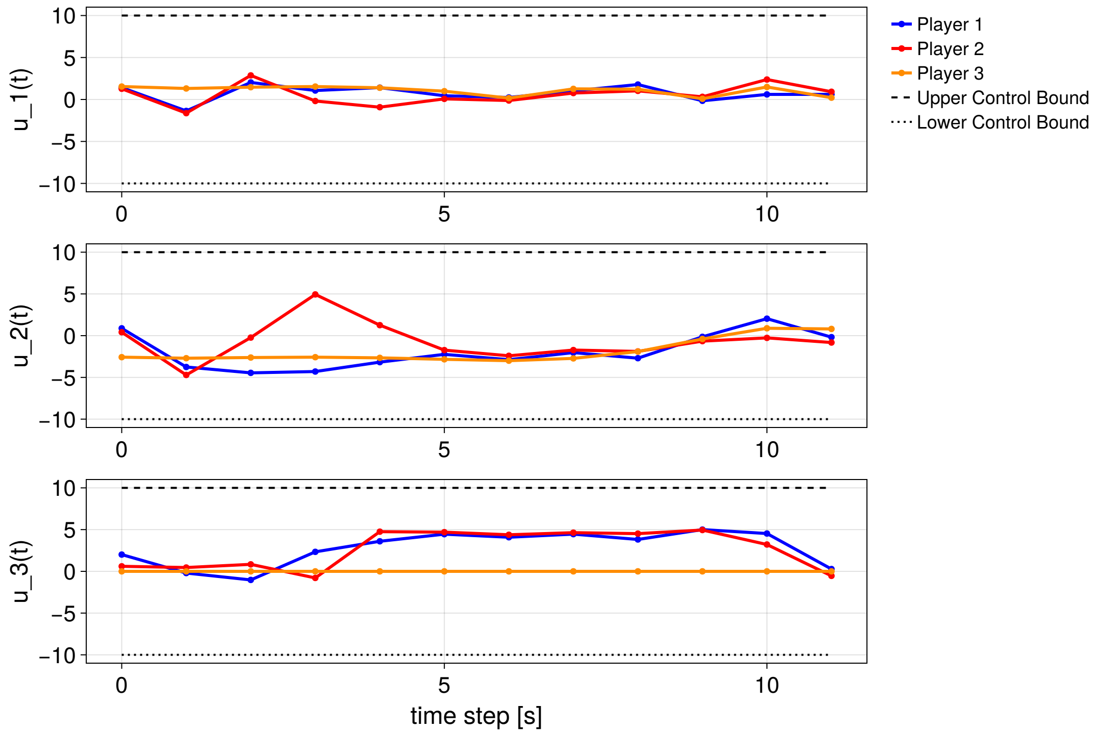
MPC step 23/25 — NOT CONVERGED (KKT error 0.214)
