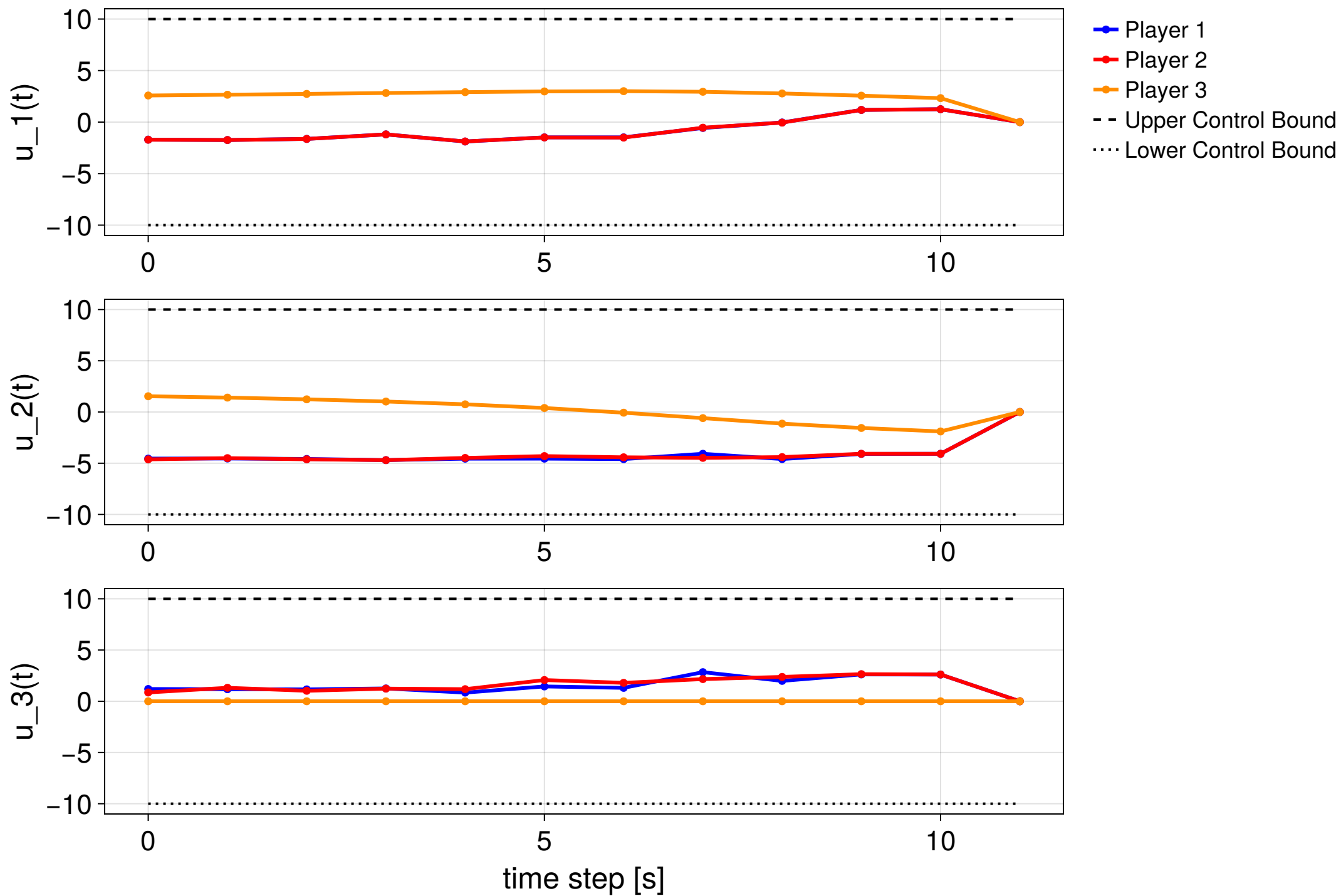
MPC step 5/25 — NOT CONVERGED (KKT error 0.0318)
