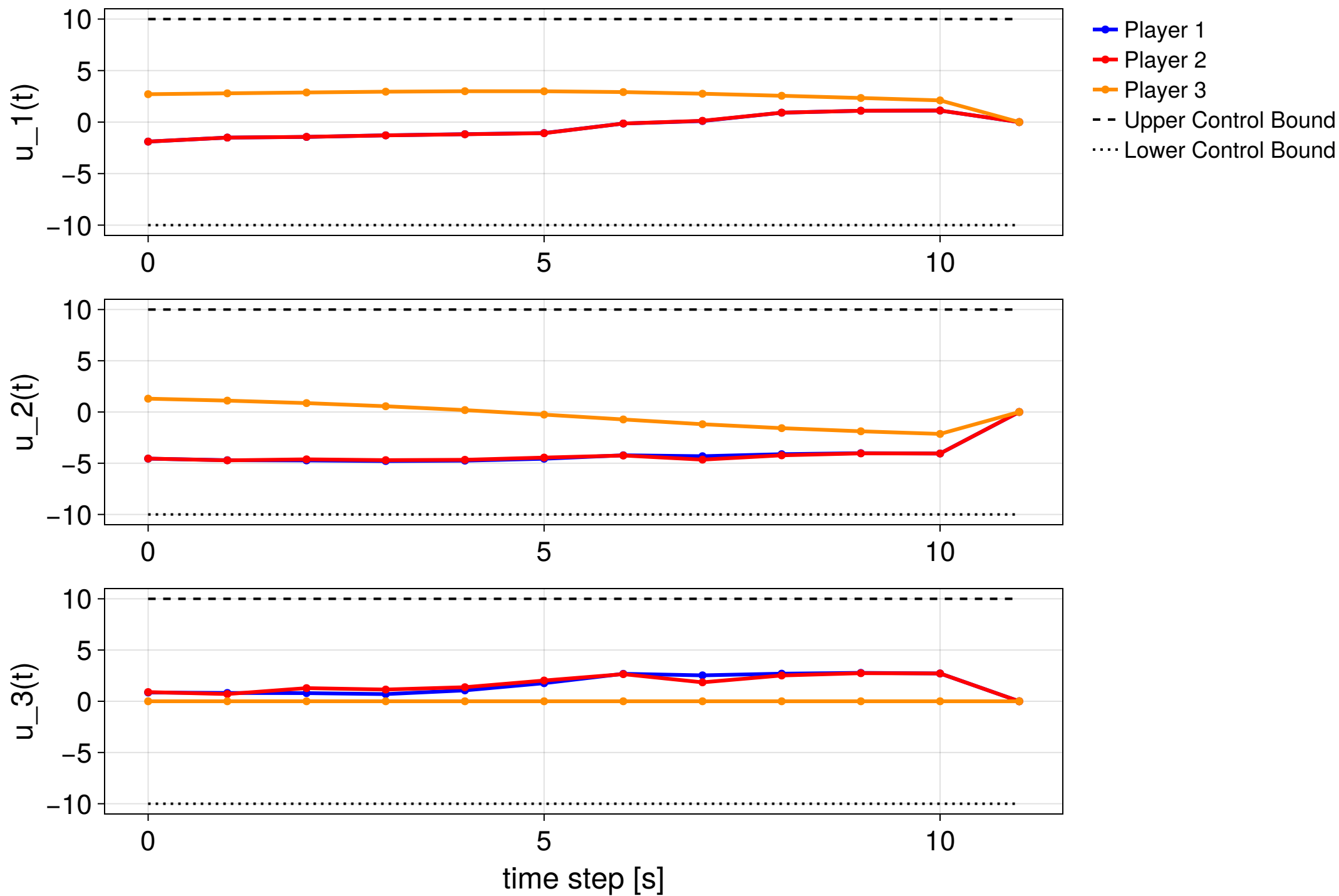
MPC step 6/25 — NOT CONVERGED (KKT error 0.427)
