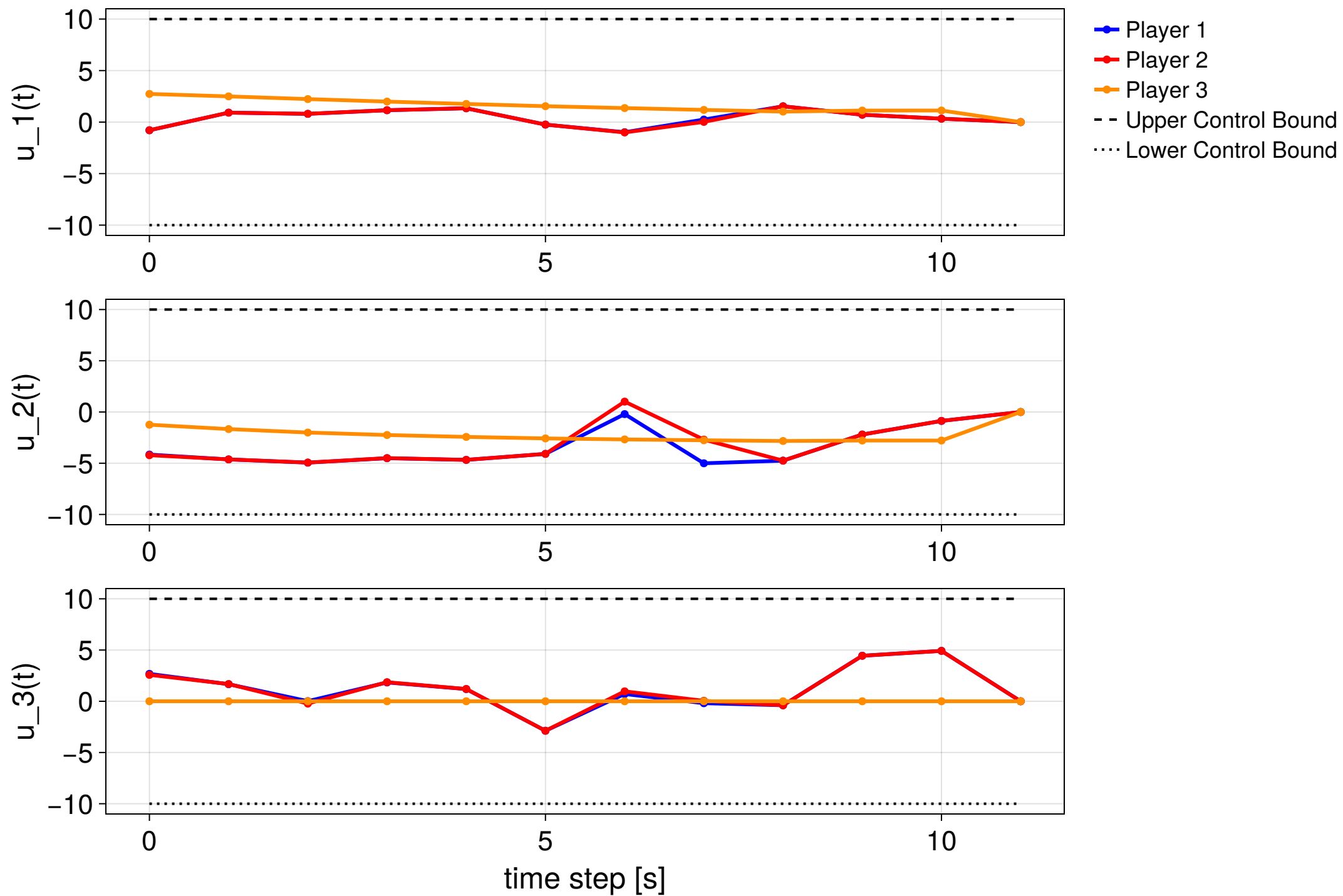
MPC step 12/20 — NOT CONVERGED (KKT error 0.769)
