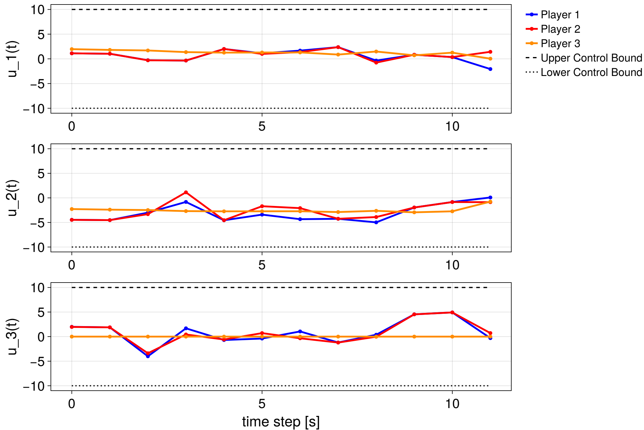
MPC step 15/20 — NOT CONVERGED (KKT error 1.16)
