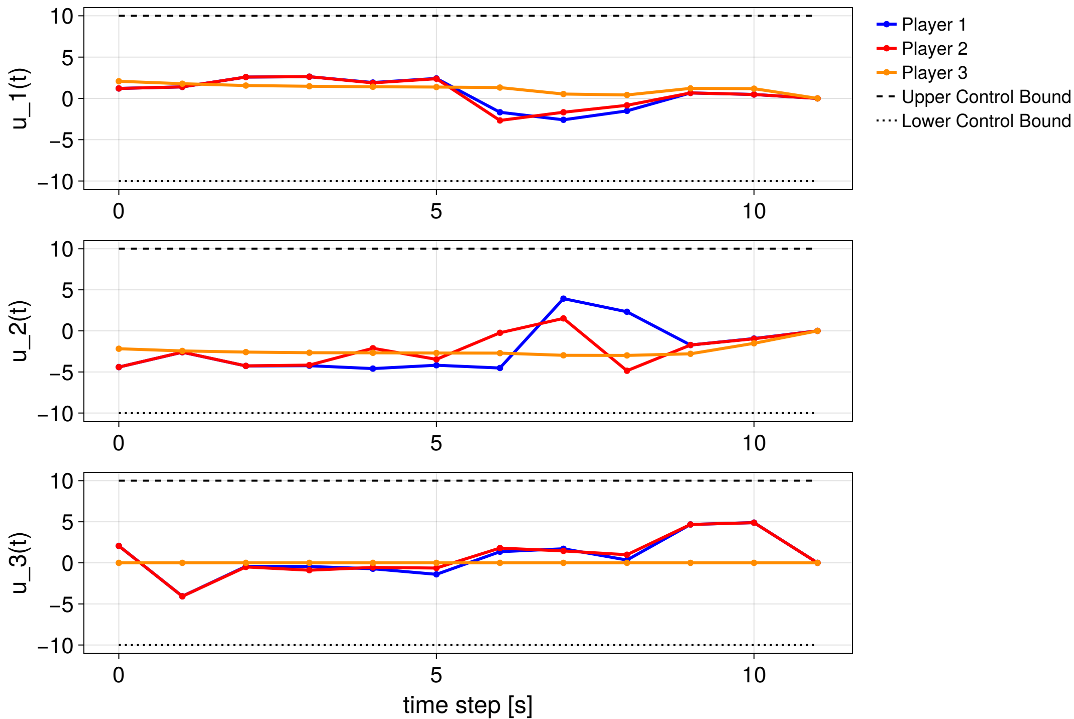
MPC step 16/20 — NOT CONVERGED (KKT error 5.39)
